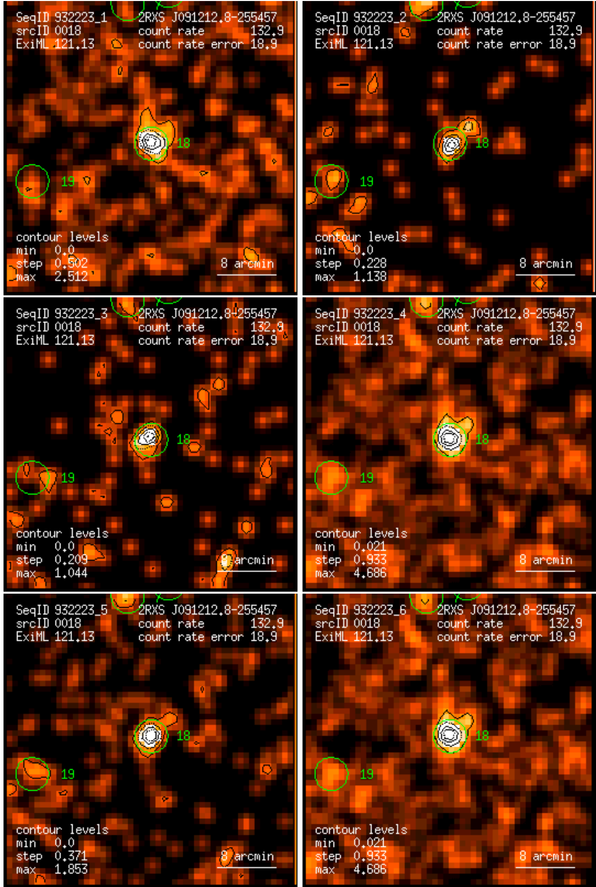
Figure 18: RASS 932223: detection 0018: band rate images, Gaussian filter: (1) PSPC channels 11 – 41, (2) 52 – 90, (3) 91 – 201, (4) 11 – 235, (5) 52 – 201, (6) 11 – 201. Broad band rates in counts/ks. Band rate contour levels in counts/ks/arcmin 2 .
