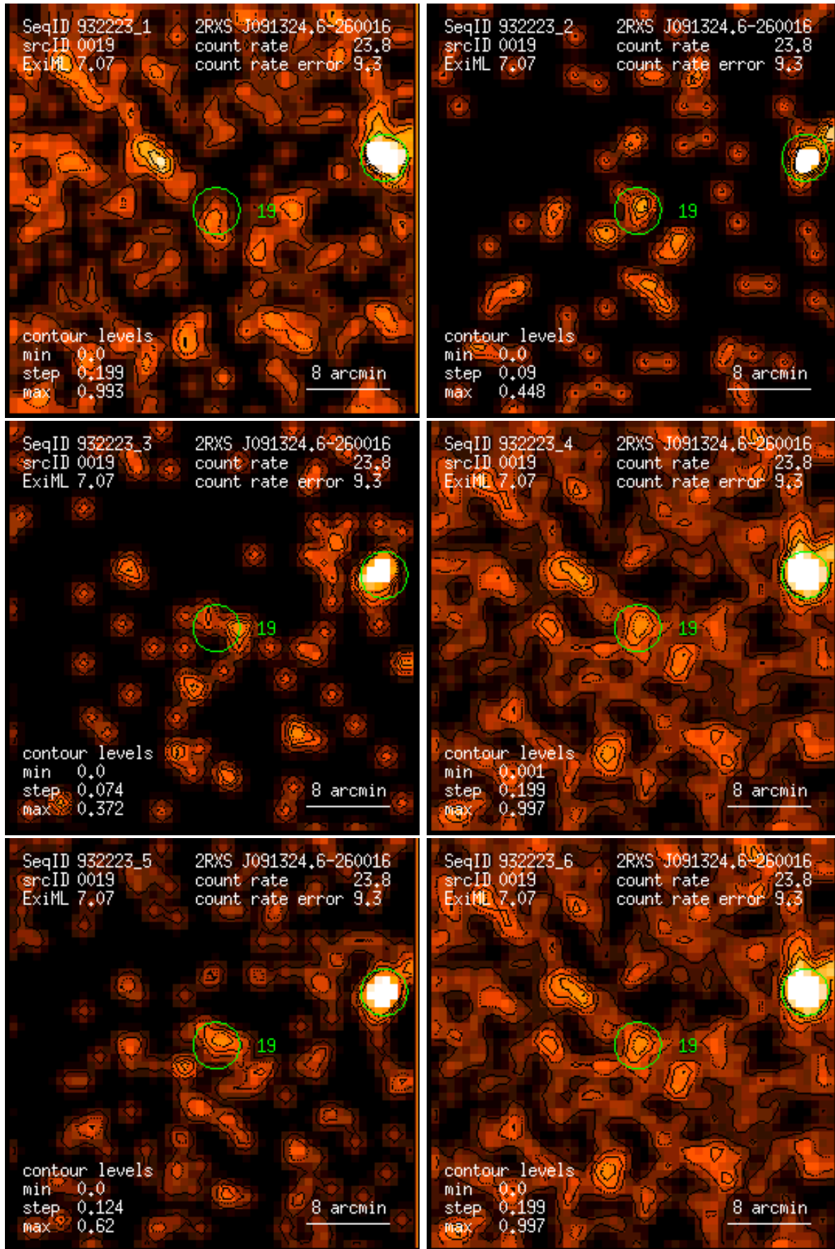
Figure 19: RASS 932223: detection 0019: band rate images, Gaussian filter: (1) PSPC channels 11 – 41, (2) 52 – 90, (3) 91 – 201, (4) 11 – 235, (5) 52 – 201, (6) 11 – 201. Broad band rates in counts/ks. Band rate contour levels in counts/ks/arcmin 2 .
