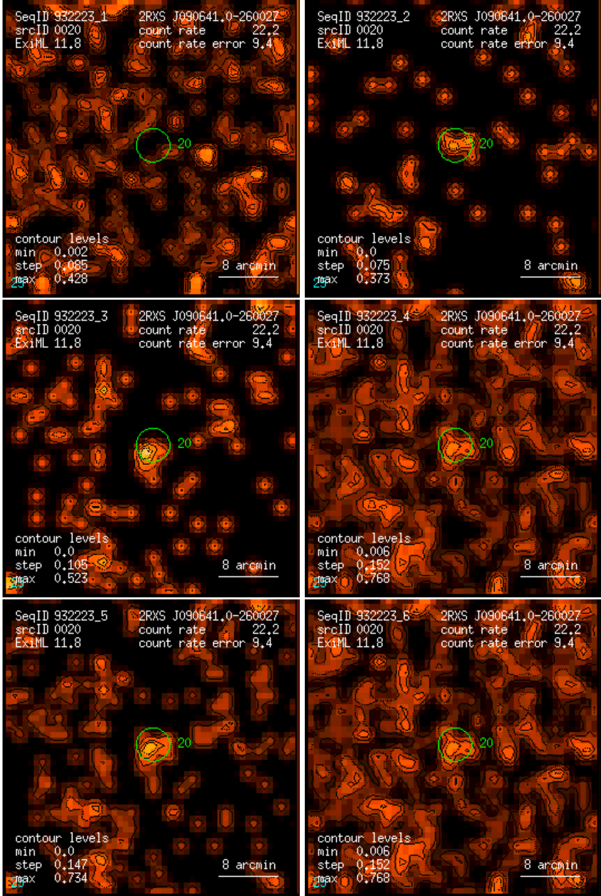
Figure 20: RASS 932223: detection 0020: band rate images, Gaussian filter: (1) PSPC channels 11 – 41, (2) 52 – 90, (3) 91 – 201, (4) 11 – 235, (5) 52 – 201, (6) 11 – 201. Broad band rates in counts/ks. Band rate contour levels in counts/ks/arcmin 2 .
