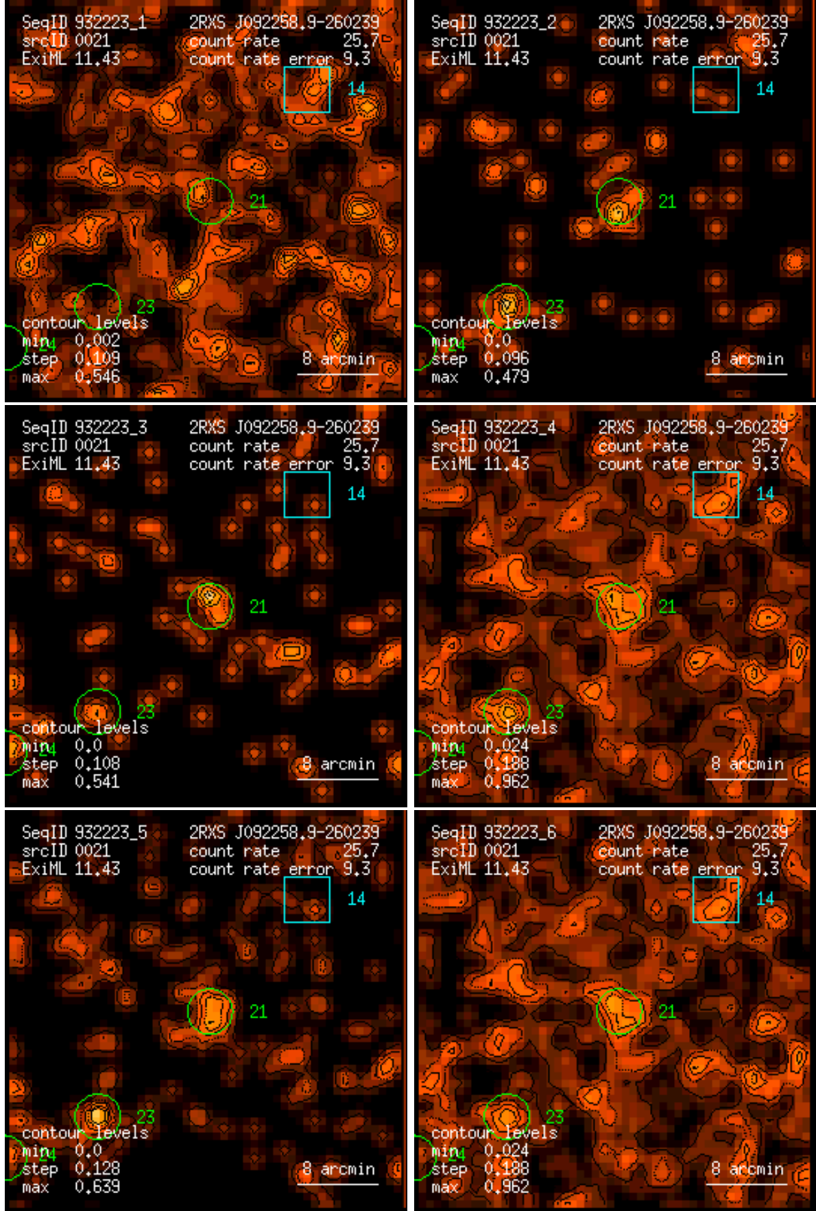
Figure 21: RASS 932223: detection 0021: band rate images, Gaussian filter: (1) PSPC channels 11 – 41, (2) 52 – 90, (3) 91 – 201, (4) 11 – 235, (5) 52 – 201, (6) 11 – 201. Broad band rates in counts/ks. Band rate contour levels in counts/ks/arcmin 2 .
