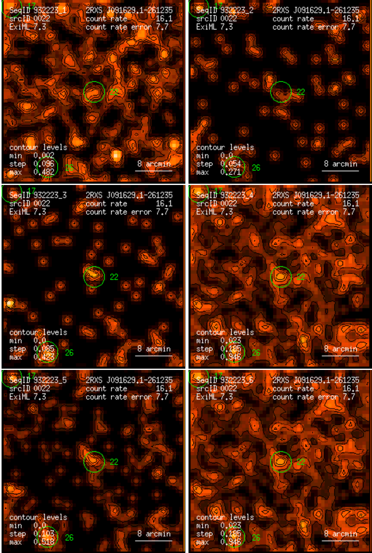
Figure 22: RASS 932223: detection 0022: band rate images, Gaussian filter: (1) PSPC channels 11 – 41, (2) 52 – 90, (3) 91 – 201, (4) 11 – 235, (5) 52 – 201, (6) 11 – 201. Broad band rates in counts/ks. Band rate contour levels in counts/ks/arcmin 2 .
