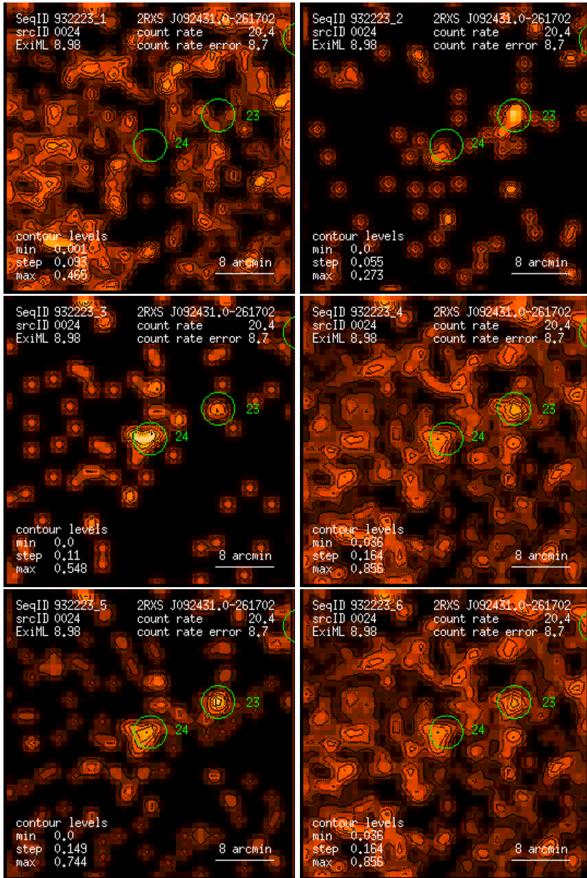
Figure 24: RASS 932223: detection 0024: band rate images, Gaussian filter: (1) PSPC channels 11 – 41, (2) 52 – 90, (3) 91 – 201, (4) 11 – 235, (5) 52 – 201, (6) 11 – 201. Broad band rates in counts/ks. Band rate contour levels in counts/ks/arcmin 2 .
