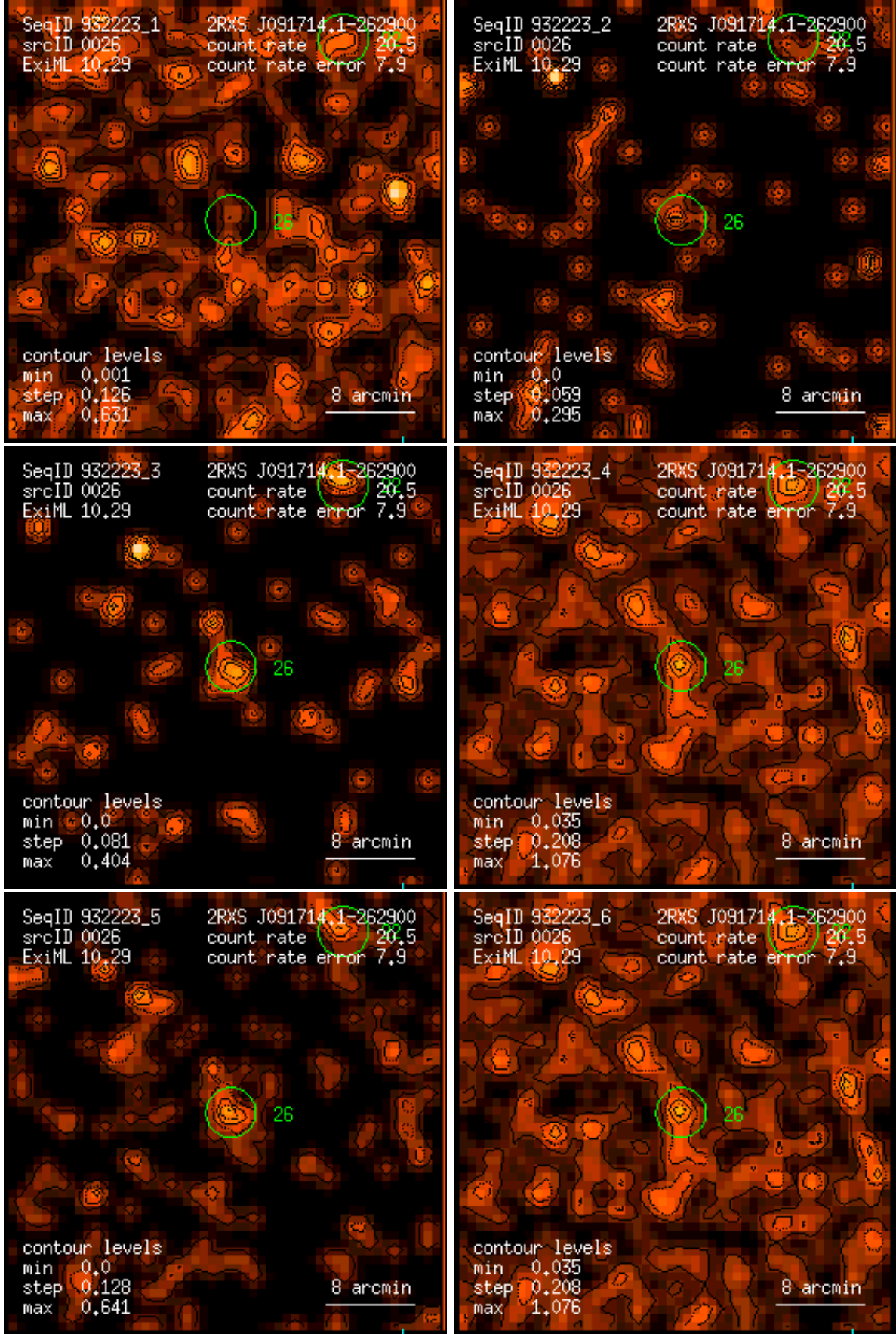
Figure 26: RASS 932223: detection 0026: band rate images, Gaussian filter: (1) PSPC channels 11 – 41, (2) 52 – 90, (3) 91 – 201, (4) 11 – 235, (5) 52 – 201, (6) 11 – 201. Broad band rates in counts/ks. Band rate contour levels in counts/ks/arcmin 2 .
