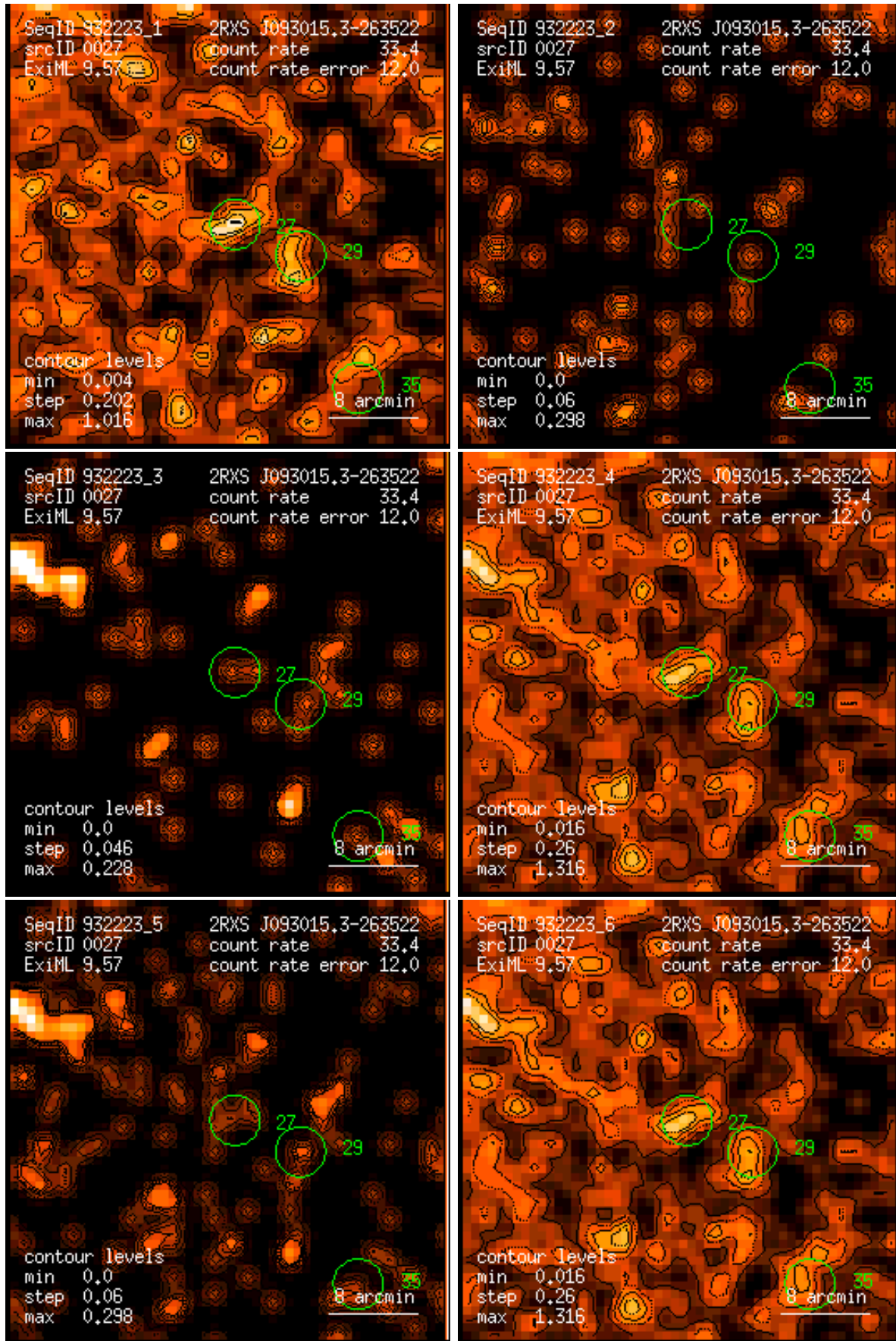
Figure 27: RASS 932223: detection 0027: band rate images, Gaussian filter: (1) PSPC channels 11 – 41, (2) 52 – 90, (3) 91 – 201, (4) 11 – 235, (5) 52 – 201, (6) 11 – 201. Broad band rates in counts/ks. Band rate contour levels in counts/ks/arcmin 2 .
