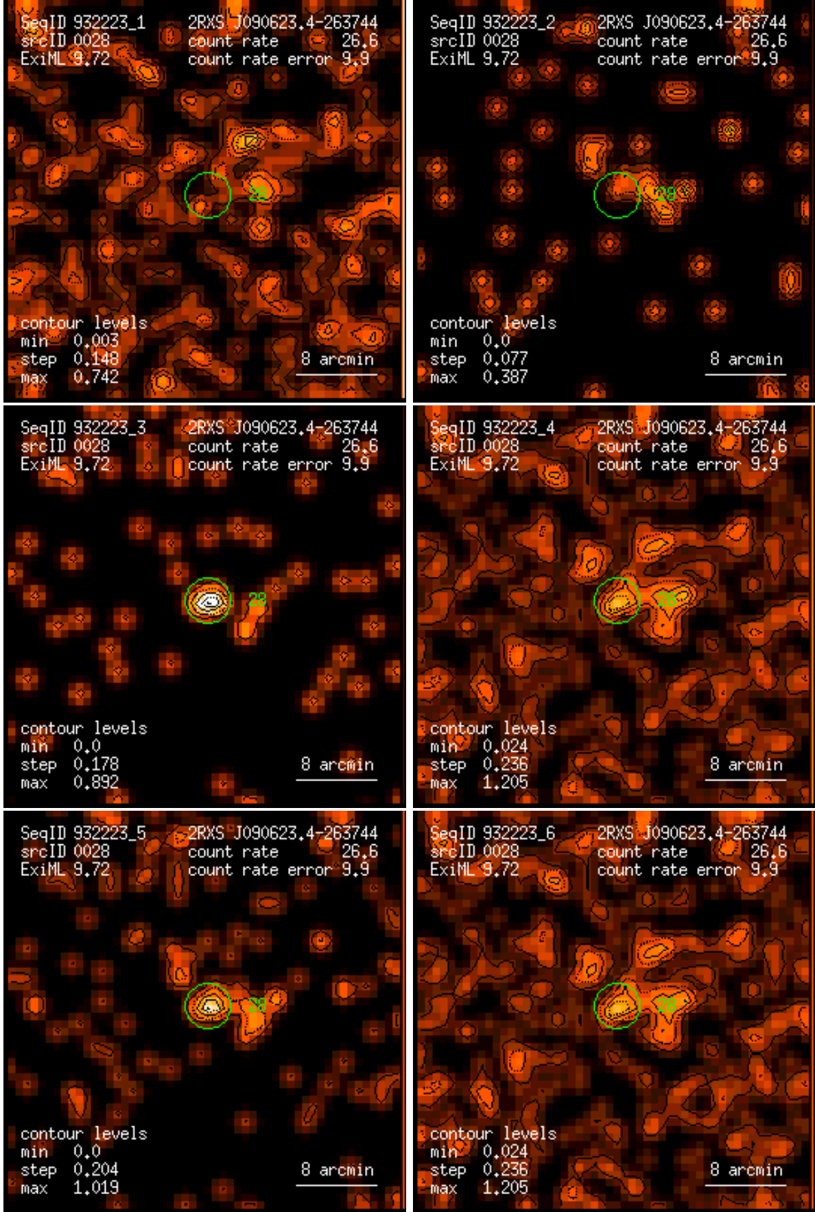
Figure 28: RASS 932223: detection 0028: band rate images, Gaussian filter: (1) PSPC channels 11 – 41, (2) 52 – 90, (3) 91 – 201, (4) 11 – 235, (5) 52 – 201, (6) 11 – 201. Broad band rates in counts/ks. Band rate contour levels in counts/ks/arcmin 2 .
