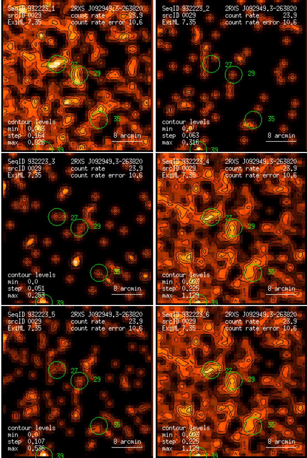
Figure 29: RASS 932223: detection 0029: band rate images, Gaussian filter: (1) PSPC channels 11 – 41, (2) 52 – 90, (3) 91 – 201, (4) 11 – 235, (5) 52 – 201, (6) 11 – 201. Broad band rates in counts/ks. Band rate contour levels in counts/ks/arcmin 2 .
