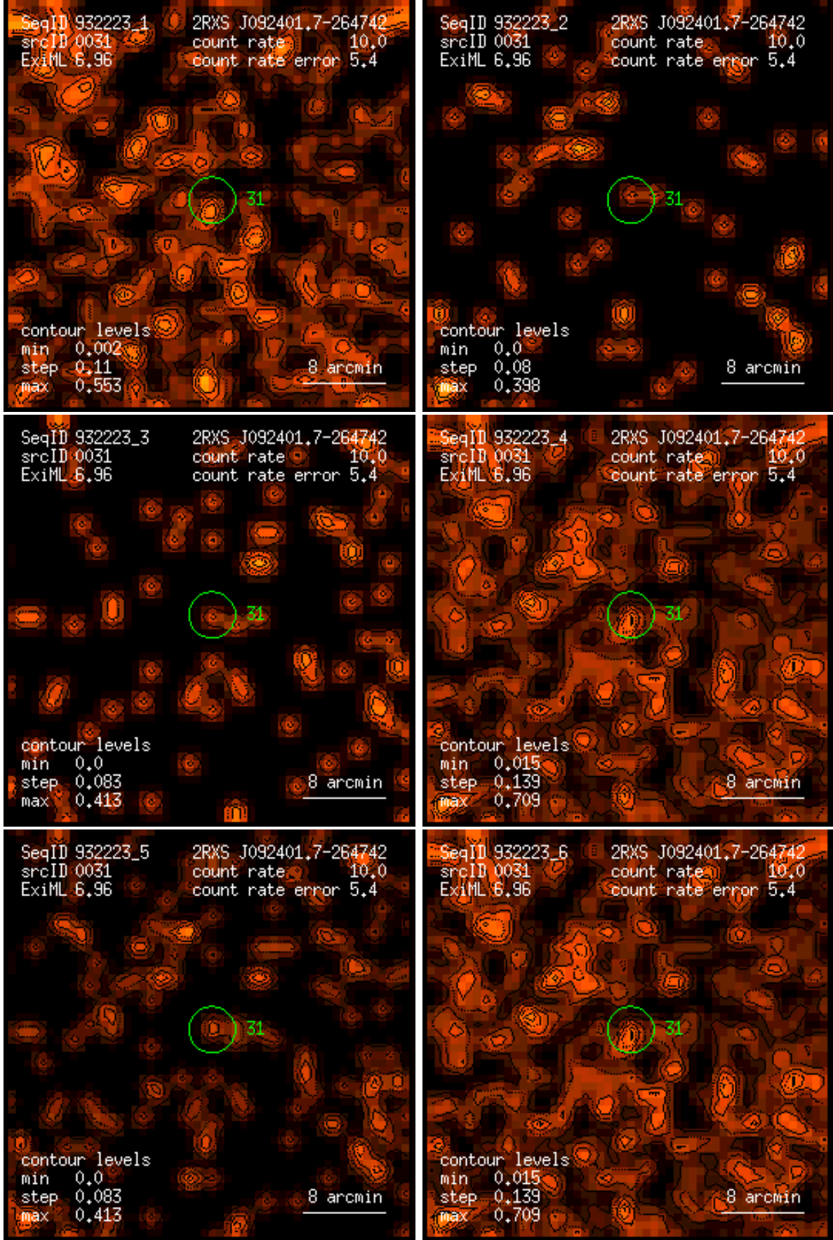
Figure 31: RASS 932223: detection 0031: band rate images, Gaussian filter: (1) PSPC channels 11 – 41, (2) 52 – 90, (3) 91 – 201, (4) 11 – 235, (5) 52 – 201, (6) 11 – 201. Broad band rates in counts/ks. Band rate contour levels in counts/ks/arcmin 2 .
