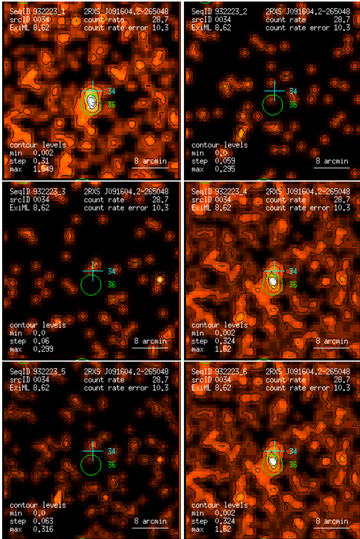
Figure 34: RASS 932223: detection 0034: band rate images, Gaussian filter: (1) PSPC channels 11 – 41, (2) 52 – 90, (3) 91 – 201, (4) 11 – 235, (5) 52 – 201, (6) 11 – 201. Broad band rates in counts/ks. Band rate contour levels in counts/ks/arcmin 2 .
