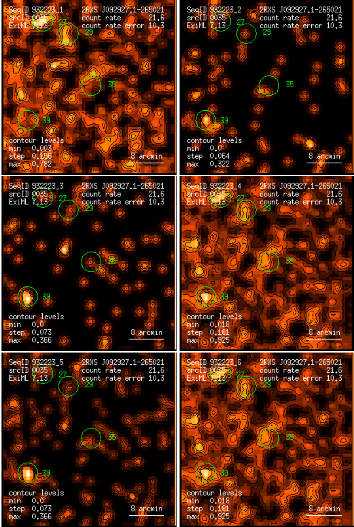
Figure 35: RASS 932223: detection 0035: band rate images, Gaussian filter: (1) PSPC channels 11 – 41, (2) 52 – 90, (3) 91 – 201, (4) 11 – 235, (5) 52 – 201, (6) 11 – 201. Broad band rates in counts/ks. Band rate contour levels in counts/ks/arcmin 2 .
