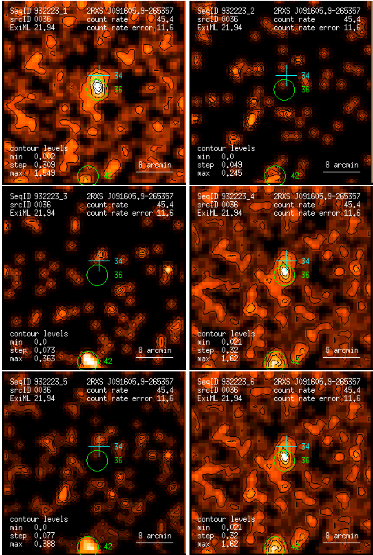
Figure 36: RASS 932223: detection 0036: band rate images, Gaussian filter: (1) PSPC channels 11 – 41, (2) 52 – 90, (3) 91 – 201, (4) 11 – 235, (5) 52 – 201, (6) 11 – 201. Broad band rates in counts/ks. Band rate contour levels in counts/ks/arcmin 2 .
