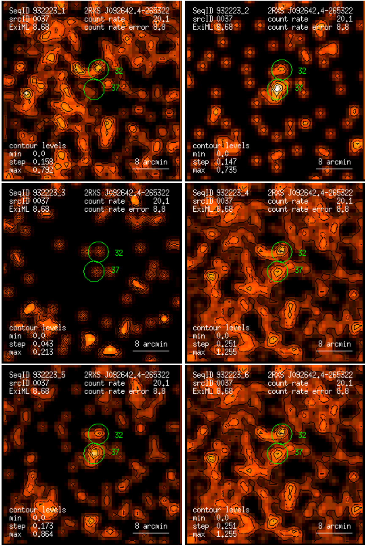
Figure 37: RASS 932223: detection 0037: band rate images, Gaussian filter: (1) PSPC channels 11 – 41, (2) 52 – 90, (3) 91 – 201, (4) 11 – 235, (5) 52 – 201, (6) 11 – 201. Broad band rates in counts/ks. Band rate contour levels in counts/ks/arcmin 2 .
