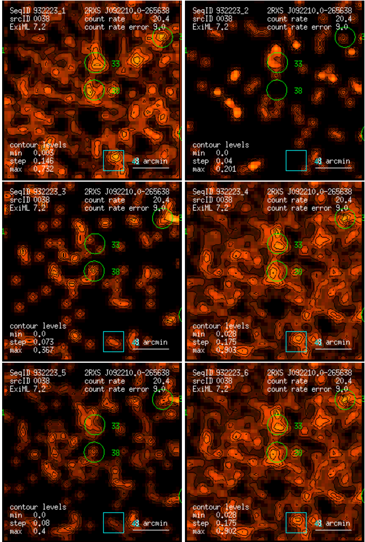
Figure 38: RASS 932223: detection 0038: band rate images, Gaussian filter: (1) PSPC channels 11 – 41, (2) 52 – 90, (3) 91 – 201, (4) 11 – 235, (5) 52 – 201, (6) 11 – 201. Broad band rates in counts/ks. Band rate contour levels in counts/ks/arcmin 2 .
