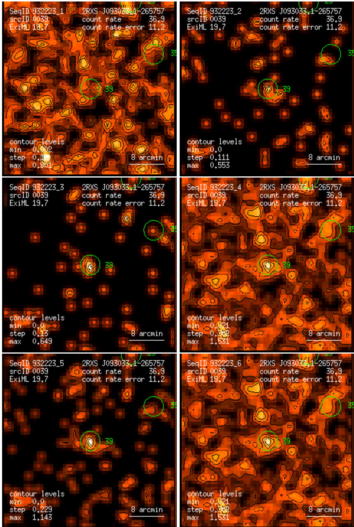
Figure 39: RASS 932223: detection 0039: band rate images, Gaussian filter: (1) PSPC channels 11 – 41, (2) 52 – 90, (3) 91 – 201, (4) 11 – 235, (5) 52 – 201, (6) 11 – 201. Broad band rates in counts/ks. Band rate contour levels in counts/ks/arcmin 2 .
