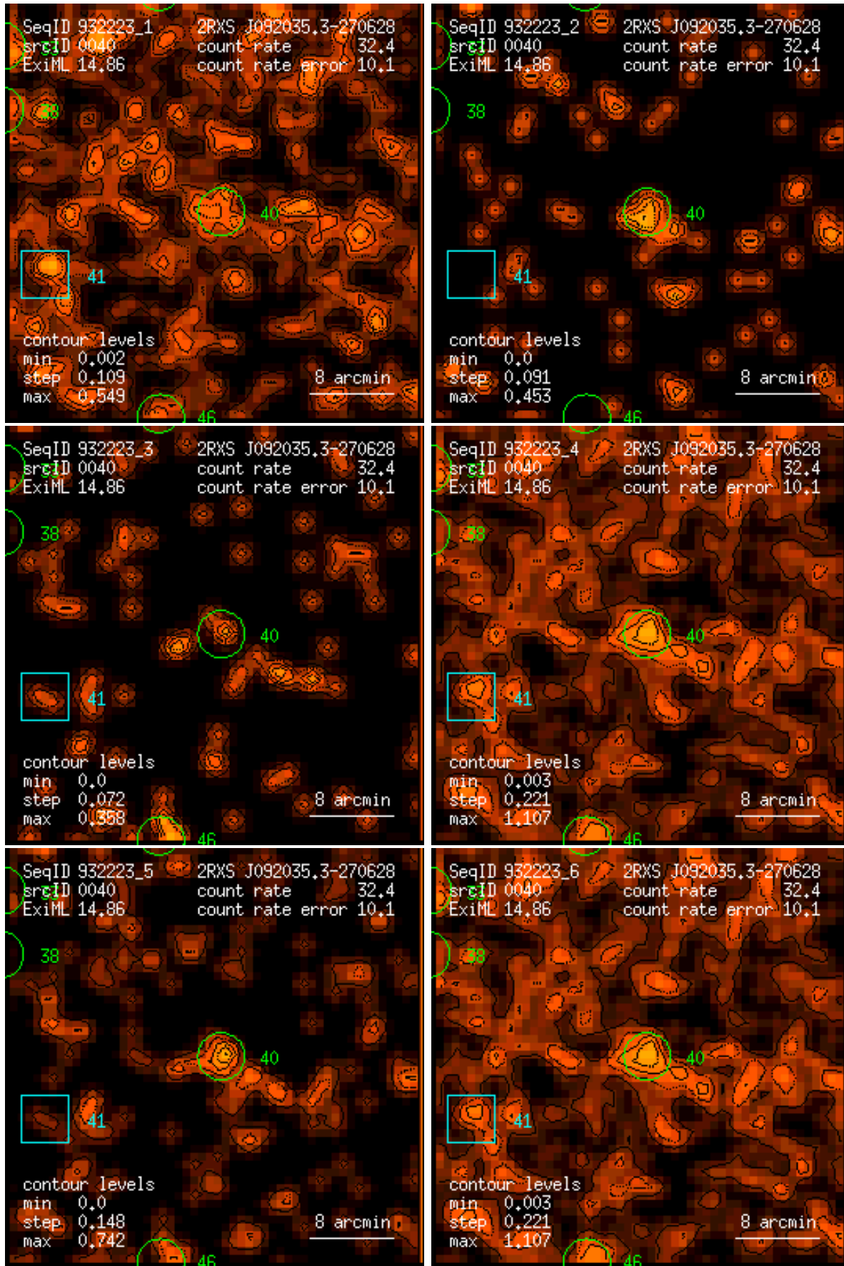
Figure 40: RASS 932223: detection 0040: band rate images, Gaussian filter: (1) PSPC channels 11 – 41, (2) 52 – 90, (3) 91 – 201, (4) 11 – 235, (5) 52 – 201, (6) 11 – 201. Broad band rates in counts/ks. Band rate contour levels in counts/ks/arcmin 2 .
