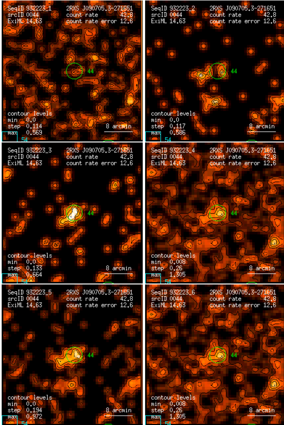
Figure 44: RASS 932223: detection 0044: band rate images, Gaussian filter: (1) PSPC channels 11 – 41, (2) 52 – 90, (3) 91 – 201, (4) 11 – 235, (5) 52 – 201, (6) 11 – 201. Broad band rates in counts/ks. Band rate contour levels in counts/ks/arcmin 2 .
