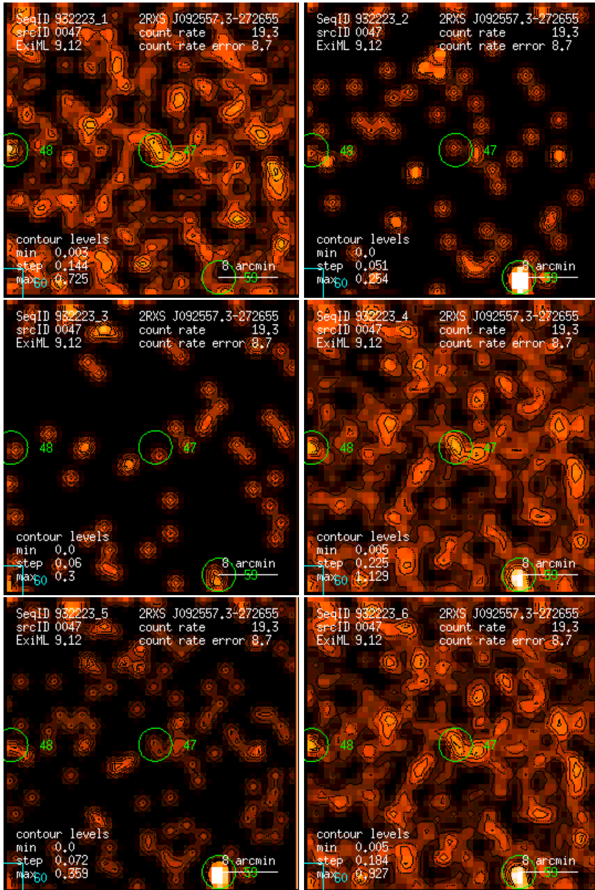
Figure 47: RASS 932223: detection 0047: band rate images, Gaussian filter: (1) PSPC channels 11 – 41, (2) 52 – 90, (3) 91 – 201, (4) 11 – 235, (5) 52 – 201, (6) 11 – 201. Broad band rates in counts/ks. Band rate contour levels in counts/ks/arcmin 2 .
