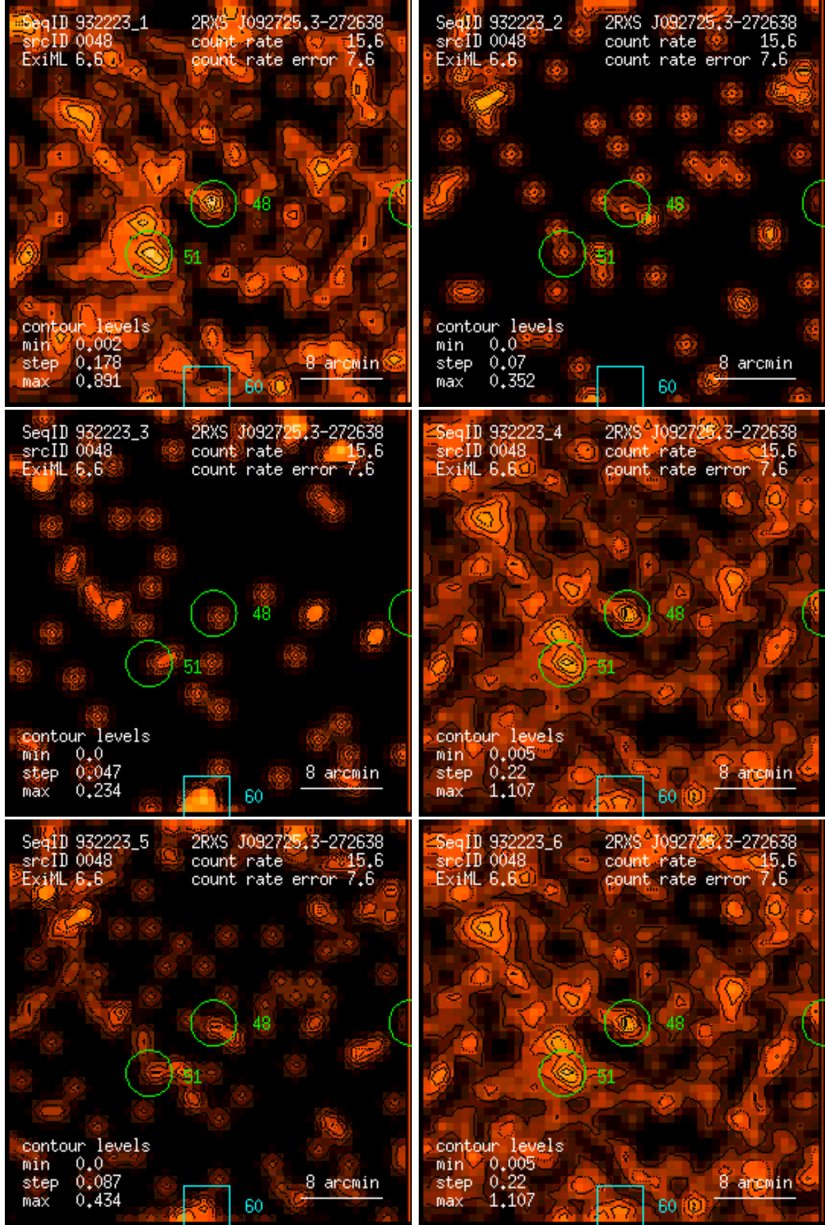
Figure 48: RASS 932223: detection 0048: band rate images, Gaussian filter: (1) PSPC channels 11 – 41, (2) 52 – 90, (3) 91 – 201, (4) 11 – 235, (5) 52 – 201, (6) 11 – 201. Broad band rates in counts/ks. Band rate contour levels in counts/ks/arcmin 2 .
