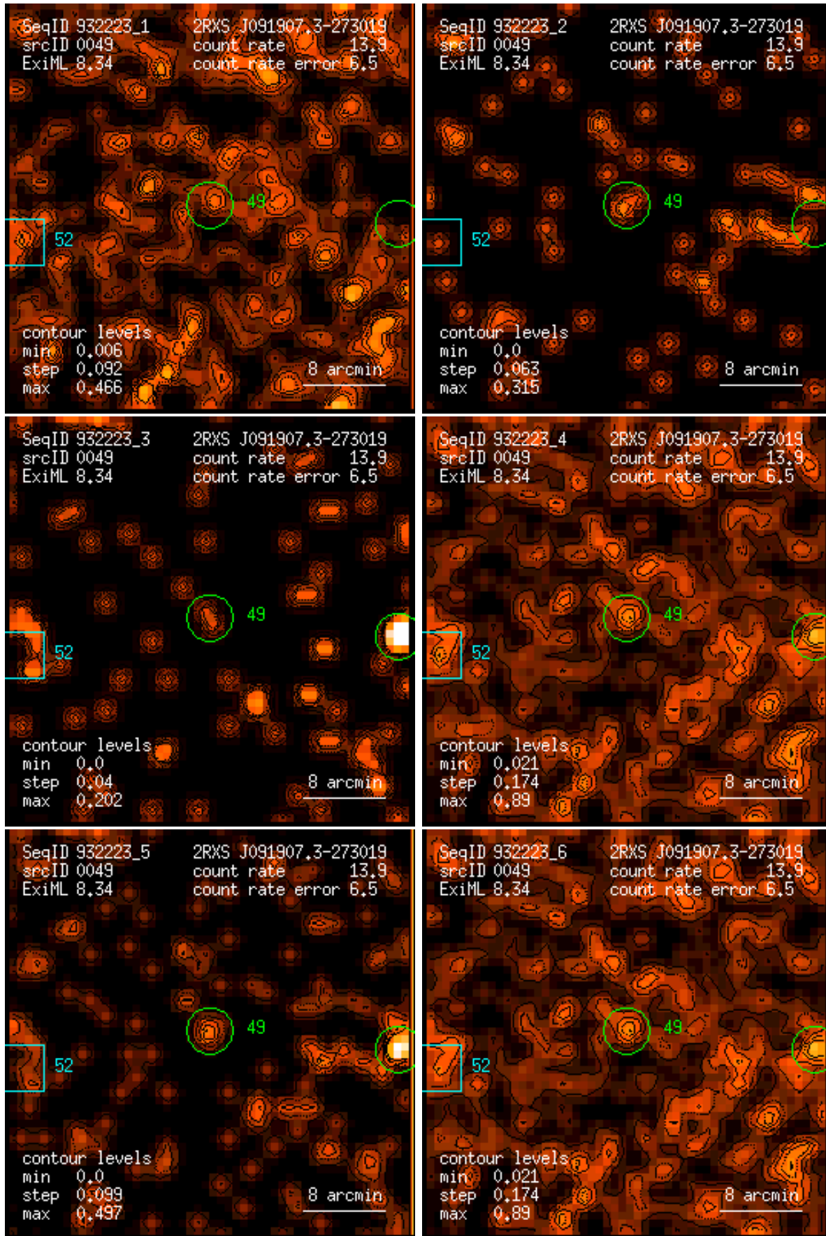
Figure 49: RASS 932223: detection 0049: band rate images, Gaussian filter: (1) PSPC channels 11 – 41, (2) 52 – 90, (3) 91 – 201, (4) 11 – 235, (5) 52 – 201, (6) 11 – 201. Broad band rates in counts/ks. Band rate contour levels in counts/ks/arcmin 2 .
