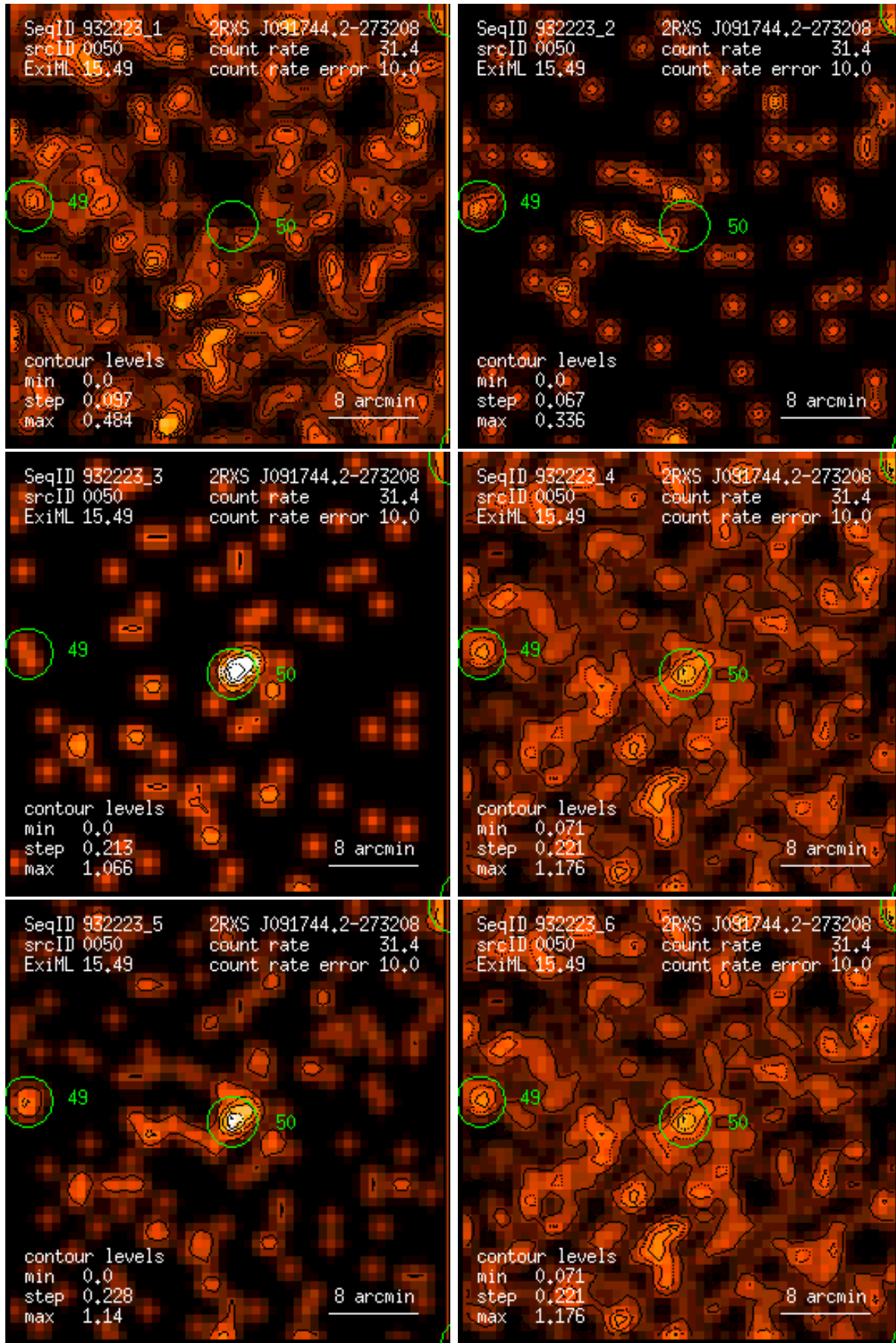
Figure 50: RASS 932223: detection 0050: band rate images, Gaussian filter: (1) PSPC channels 11 – 41, (2) 52 – 90, (3) 91 – 201, (4) 11 – 235, (5) 52 – 201, (6) 11 – 201. Broad band rates in counts/ks. Band rate contour levels in counts/ks/arcmin 2 .
