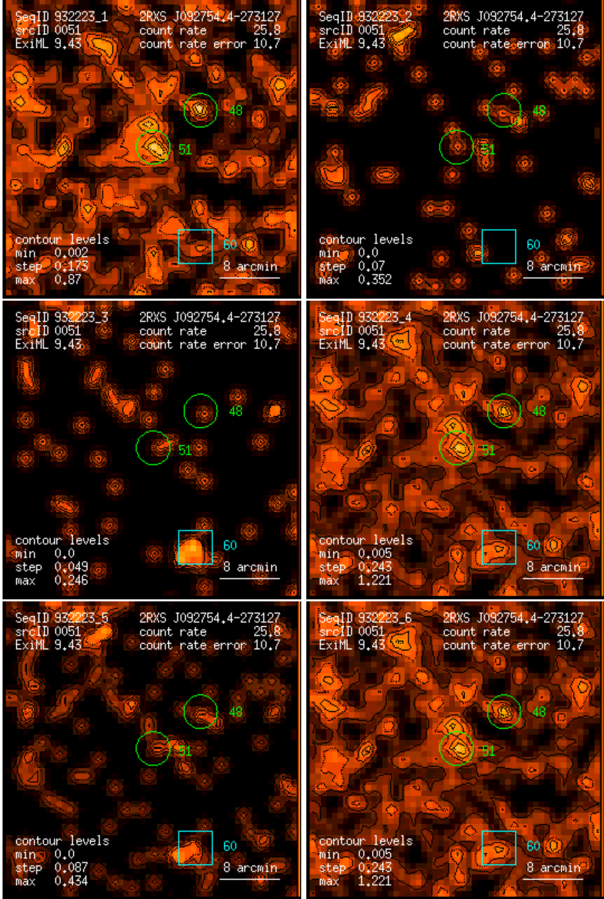
Figure 51: RASS 932223: detection 0051: band rate images, Gaussian filter: (1) PSPC channels 11 – 41, (2) 52 – 90, (3) 91 – 201, (4) 11 – 235, (5) 52 – 201, (6) 11 – 201. Broad band rates in counts/ks. Band rate contour levels in counts/ks/arcmin 2 .
