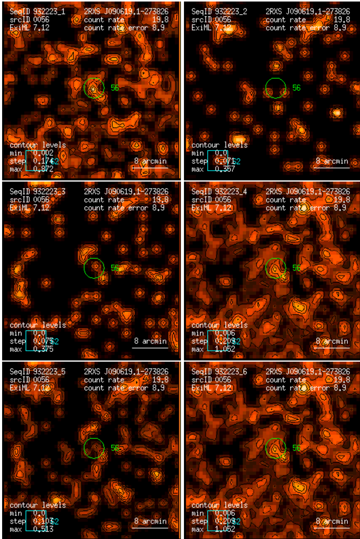
Figure 56: RASS 932223: detection 0056: band rate images, Gaussian filter: (1) PSPC channels 11 – 41, (2) 52 – 90, (3) 91 – 201, (4) 11 – 235, (5) 52 – 201, (6) 11 – 201. Broad band rates in counts/ks. Band rate contour levels in counts/ks/arcmin 2 .
