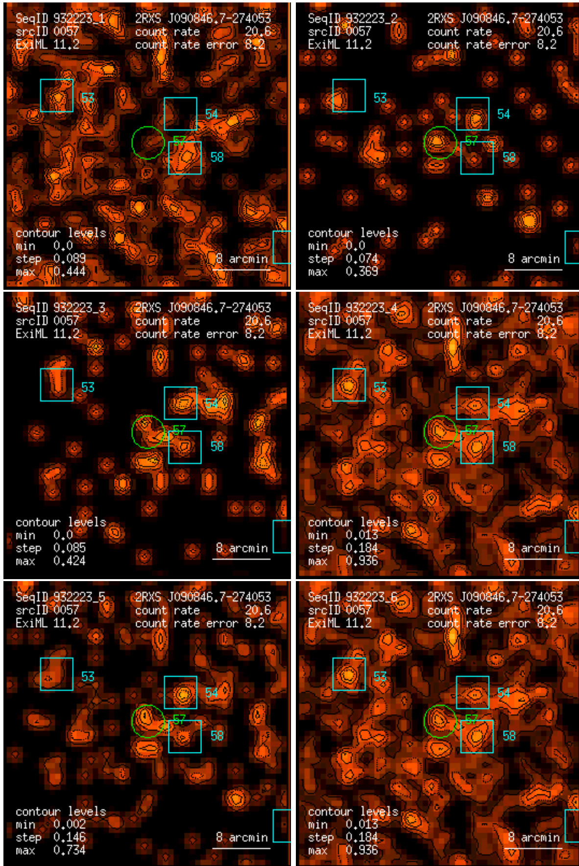
Figure 57: RASS 932223: detection 0057: band rate images, Gaussian filter: (1) PSPC channels 11 – 41, (2) 52 – 90, (3) 91 – 201, (4) 11 – 235, (5) 52 – 201, (6) 11 – 201. Broad band rates in counts/ks. Band rate contour levels in counts/ks/arcmin 2 .
