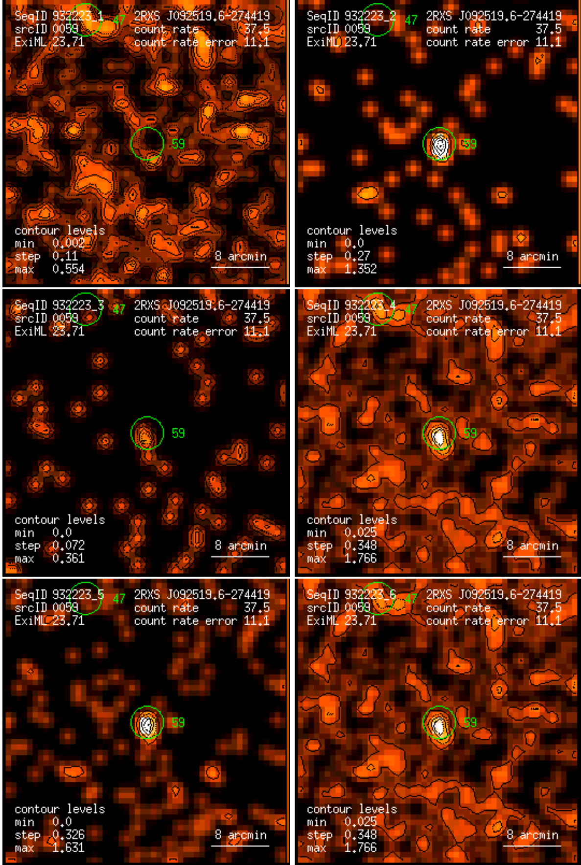
Figure 59: RASS 932223: detection 0059: band rate images, Gaussian filter: (1) PSPP channels 11 – 41, (2) 52 – 90, (3) 91 – 201, (4) 11 – 235, (5) 52 – 201, (6) 11 – 201. Broad band rates in counts/ks. Band rate contour levels in counts/ks/arcmin 2 .
