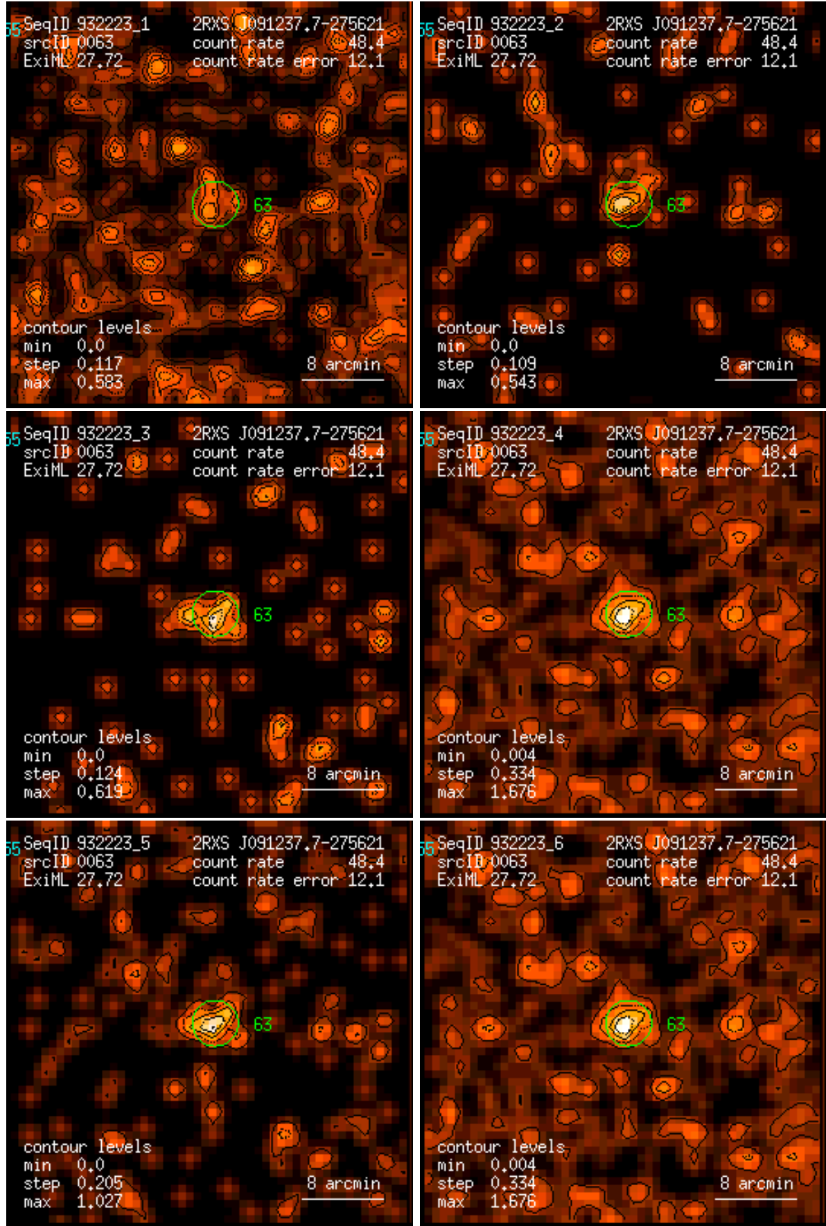
Figure 63: RASS 932223: detection 0063: band rate images, Gaussian filter: (1) PSPC channels 11 – 41, (2) 52 – 90, (3) 91 – 201, (4) 11 – 235, (5) 52 – 201, (6) 11 – 201. Broad band rates in counts/ks. Band rate contour levels in counts/ks/arcmin 2 .
