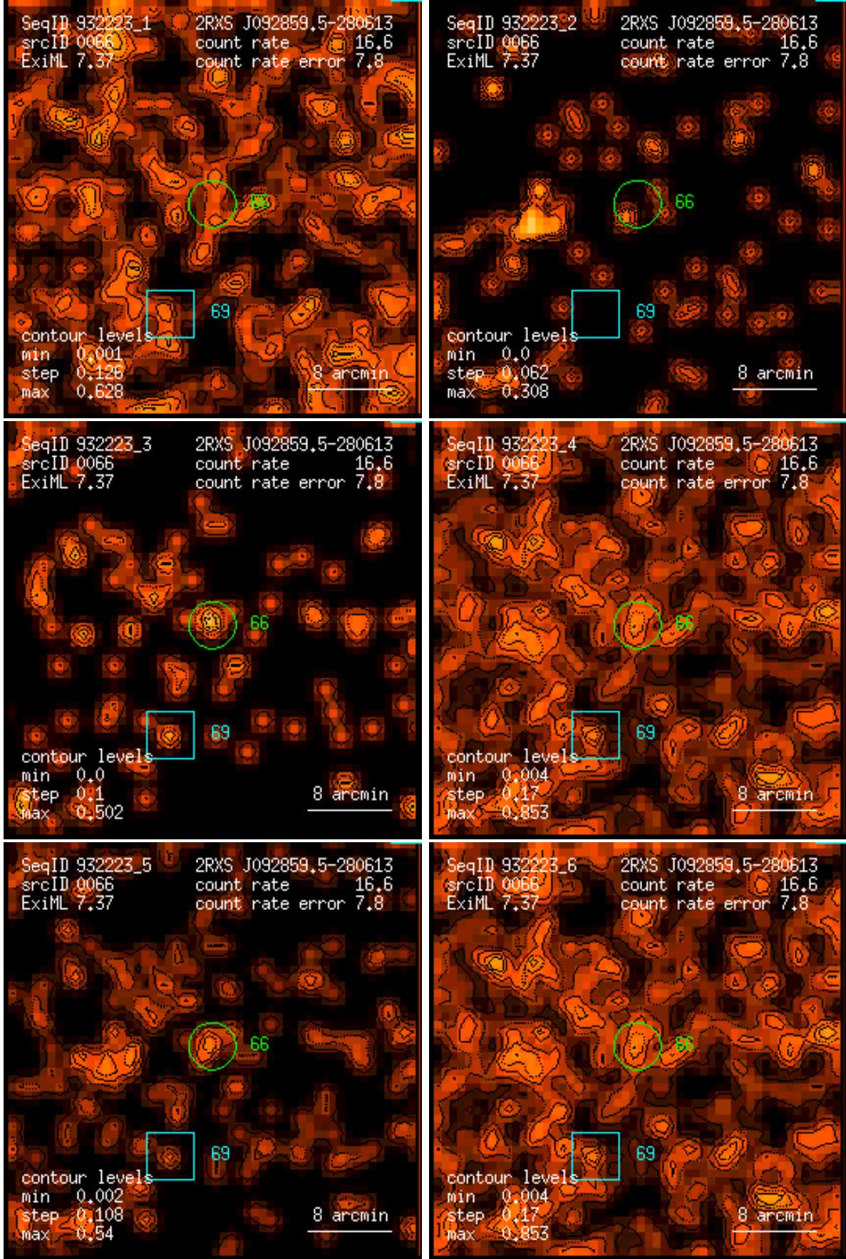
Figure 66: RASS 932223: detection 0066: band rate images, Gaussian filter: (1) PSPC channels 11 – 41, (2) 52 – 90, (3) 91 – 201, (4) 11 – 235, (5) 52 – 201, (6) 11 – 201. Broad band rates in counts/ks. Band rate contour levels in counts/ks/arcmin 2 .
