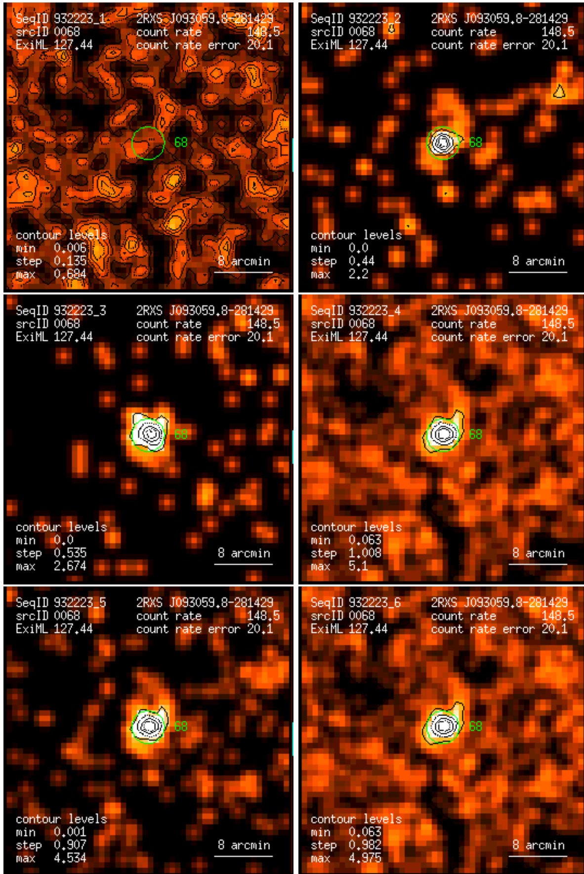
Figure 68: RASS 932223: detection 0068: band rate images, Gaussian filter: (1) PSPC channels 11 – 41, (2) 52 – 90, (3) 91 – 201, (4) 11 – 235, (5) 52 – 201, (6) 11 – 201. Broad band rates in counts/ks. Band rate contour levels in counts/ks/arcmin 2 .
