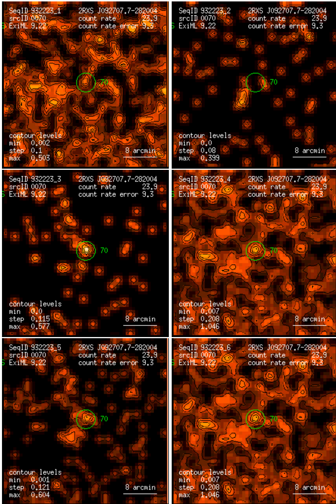
Figure 70: RASS 932223: detection 0070: band rate images, Gaussian filter: (1) PSPC channels 11 – 41, (2) 52 – 90, (3) 91 – 201, (4) 11 – 235, (5) 52 – 201, (6) 11 – 201. Broad band rates in counts/ks. Band rate contour levels in counts/ks/arcmin 2 .
