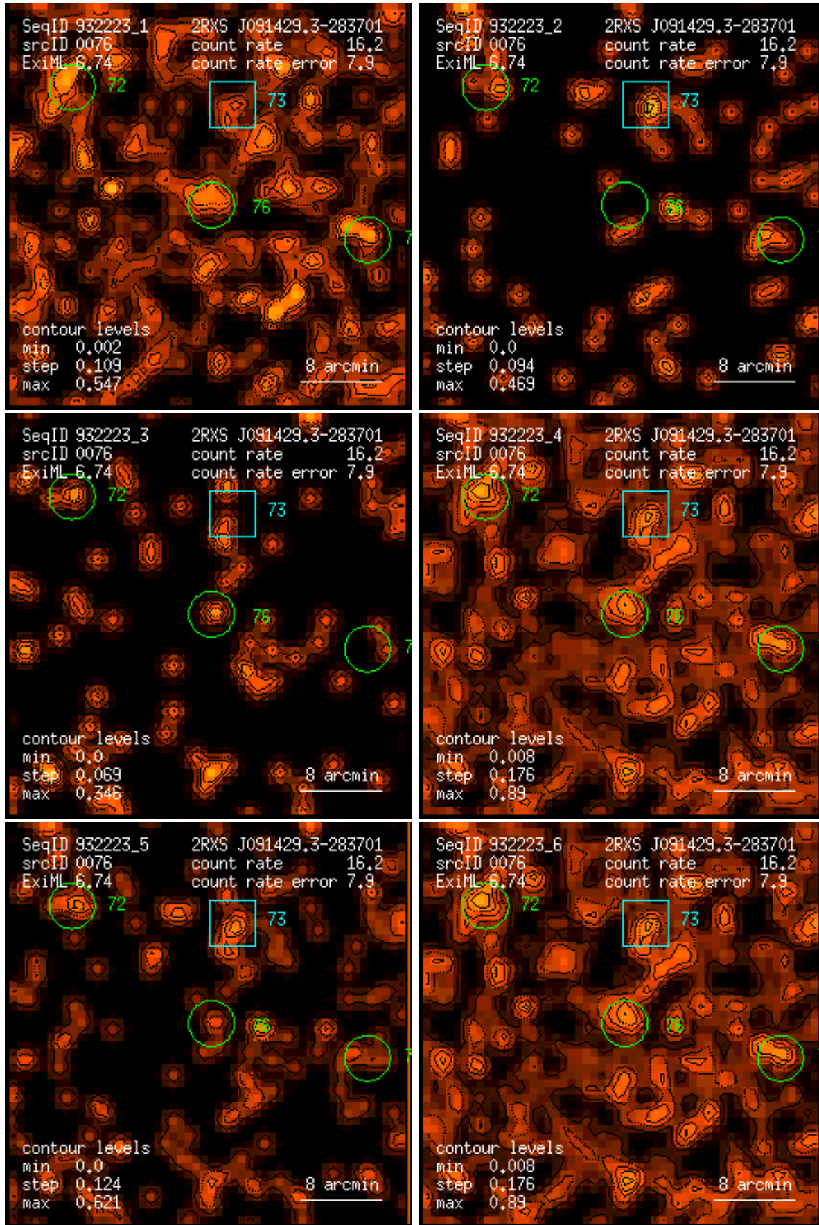
Figure 76: RASS 932223: detection 0076: band rate images, Gaussian filter: (1) PSPC channels 11 – 41, (2) 52 – 90, (3) 91 – 201, (4) 11 – 235, (5) 52 – 201, (6) 11 – 201. Broad band rates in counts/ks. Band rate contour levels in counts/ks/arcmin 2 .
