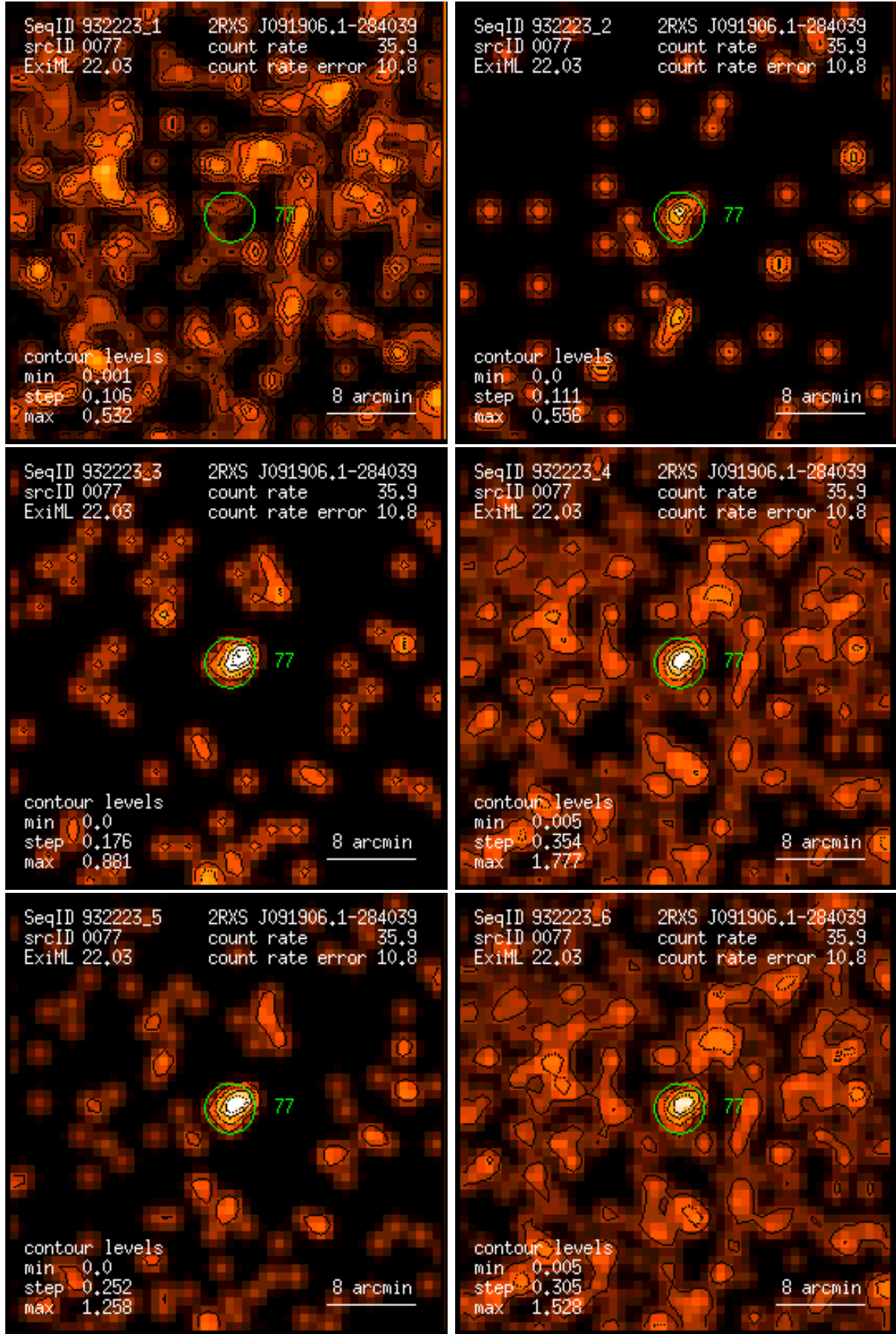
Figure 77: RASS 932223: detection 0077: band rate images, Gaussian filter: (1) PSPC channels 11 – 41, (2) 52 – 90, (3) 91 – 201, (4) 11 – 235, (5) 52 – 201, (6) 11 – 201. Broad band rates in counts/ks. Band rate contour levels in counts/ks/arcmin 2 .
