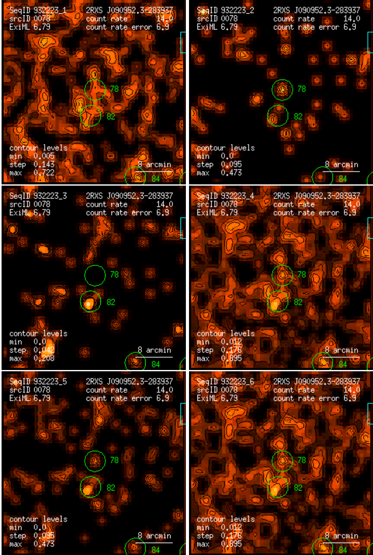
Figure 78: RASS 932223: detection 0078: band rate images, Gaussian filter: (1) PSPC channels 11 – 41, (2) 52 – 90, (3) 91 – 201, (4) 11 – 235, (5) 52 – 201, (6) 11 – 201. Broad band rates in counts/ks. Band rate contour levels in counts/ks/arcmin 2 .
