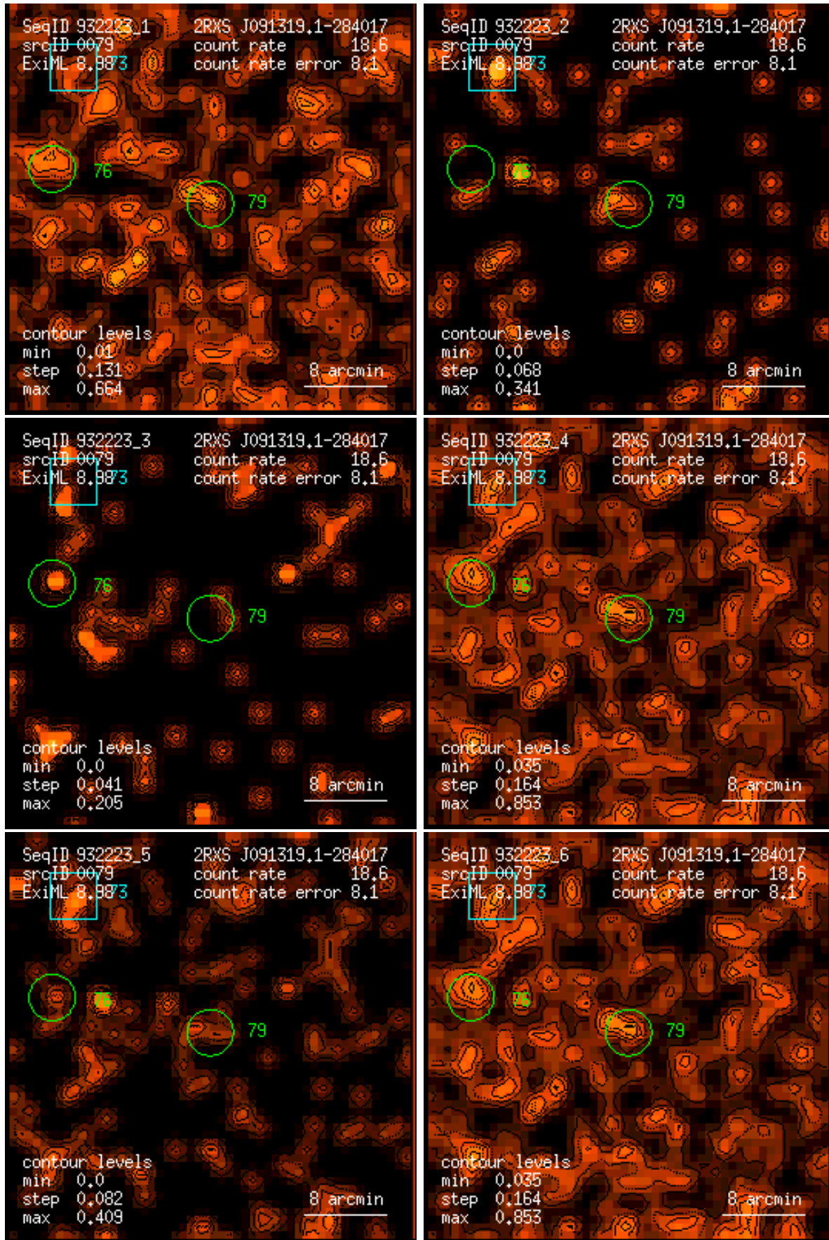
Figure 79: RASS 932223: detection 0079: band rate images, Gaussian filter: (1) PSPC channels 11 – 41, (2) 52 – 90, (3) 91 – 201, (4) 11 – 235, (5) 52 – 201, (6) 11 – 201. Broad band rates in counts/ks. Band rate contour levels in counts/ks/arcmin 2 .
