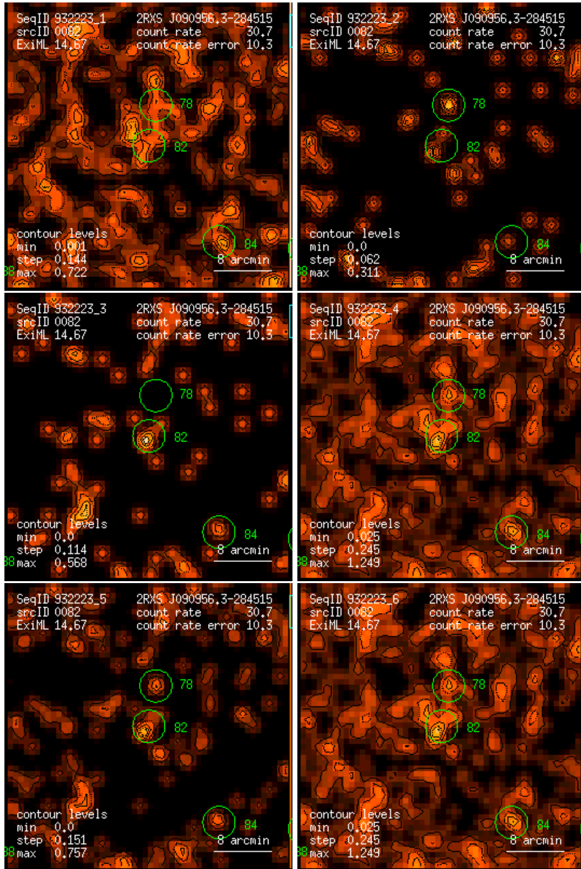
Figure 82: RASS 932223: detection 0082: band rate images, Gaussian filter: (1) PSPC channels 11 – 41, (2) 52 – 90, (3) 91 – 201, (4) 11 – 235, (5) 52 – 201, (6) 11 – 201. Broad band rates in counts/ks. Band rate contour levels in counts/ks/arcmin 2 .
