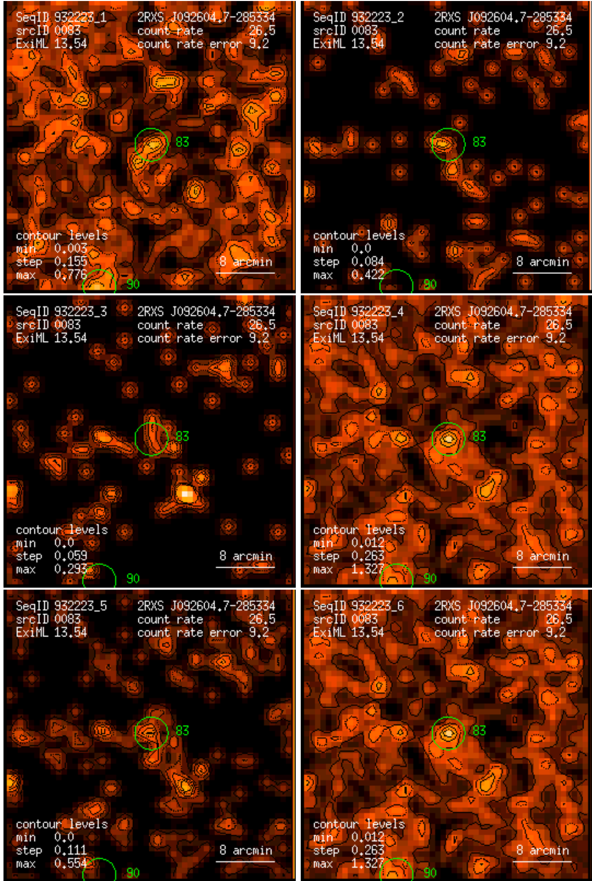
Figure 83: RASS 932223: detection 0083: band rate images, Gaussian filter: (1) PSPC channels 11 – 41, (2) 52 – 90, (3) 91 – 201, (4) 11 – 235, (5) 52 – 201, (6) 11 – 201. Broad band rates in counts/ks. Band rate contour levels in counts/ks/arcmin 2 .
