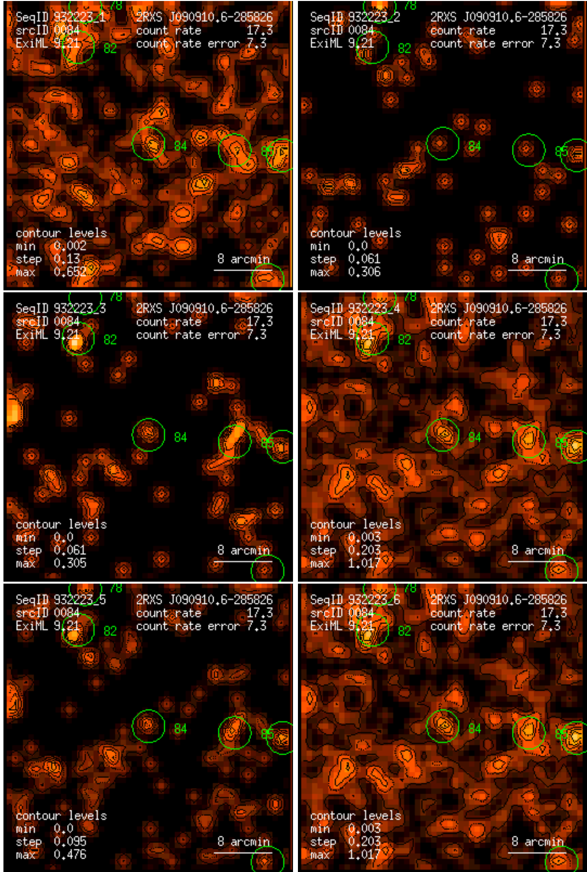
Figure 84: RASS 932223: detection 0084: band rate images, Gaussian filter: (1) PSPC channels 11 – 41, (2) 52 – 90, (3) 91 – 201, (4) 11 – 235, (5) 52 – 201, (6) 11 – 201. Broad band rates in counts/ks. Band rate contour levels in counts/ks/arcmin 2 .
