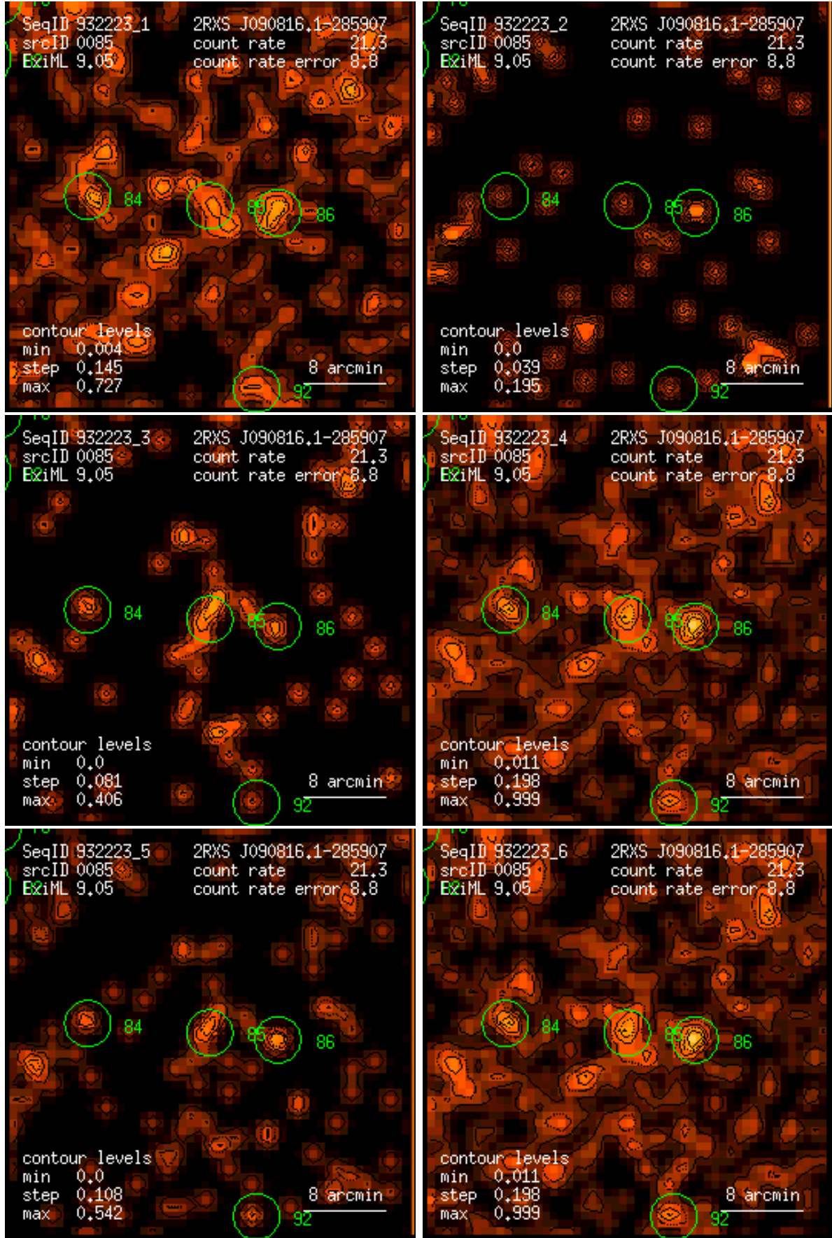
Figure 85: RASS 932223: detection 0085: band rate images, Gaussian filter: (1) PSPC channels 11 – 41, (2) 52 – 90, (3) 91 – 201, (4) 11 – 235, (5) 52 – 201, (6) 11 – 201. Broad band rates in counts/ks. Band rate contour levels in counts/ks/arcmin 2 .
