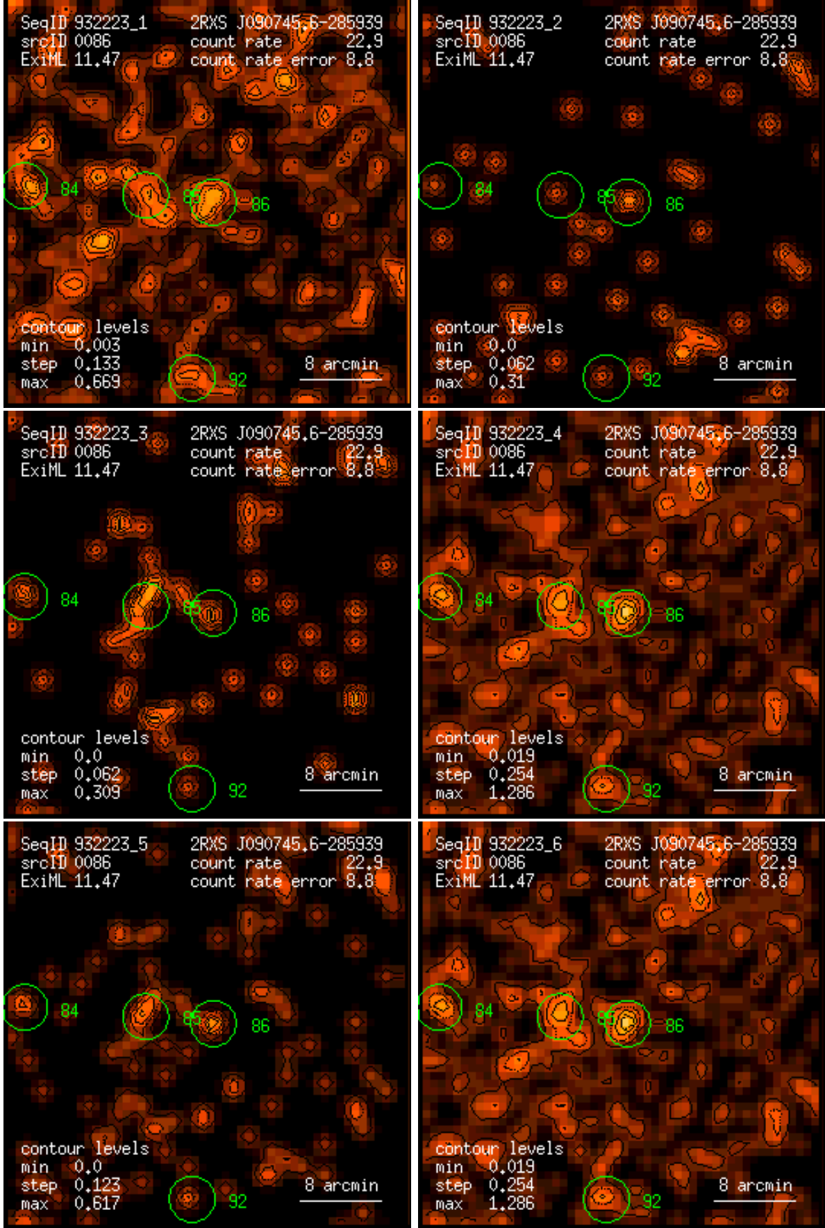
Figure 86: RASS 932223: detection 0086: band rate images, Gaussian filter: (1) PSPC channels 11 – 41, (2) 52 – 90, (3) 91 – 201, (4) 11 – 235, (5) 52 – 201, (6) 11 – 201. Broad band rates in counts/ks. Band rate contour levels in counts/ks/arcmin 2 .
