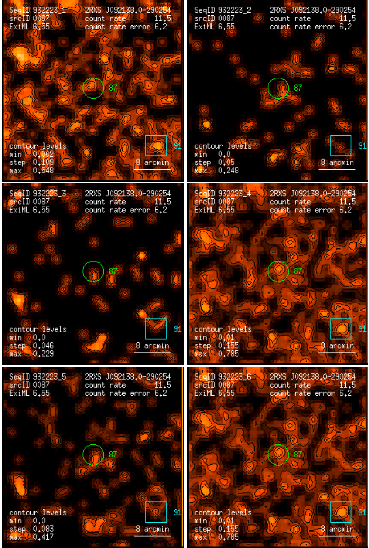
Figure 87: RASS 932223: detection 0087: band rate images, Gaussian filter: (1) PSPC channels 11 – 41, (2) 52 – 90, (3) 91 – 201, (4) 11 – 235, (5) 52 – 201, (6) 11 – 201. Broad band rates in counts/ks. Band rate contour levels in counts/ks/arcmin 2 .
