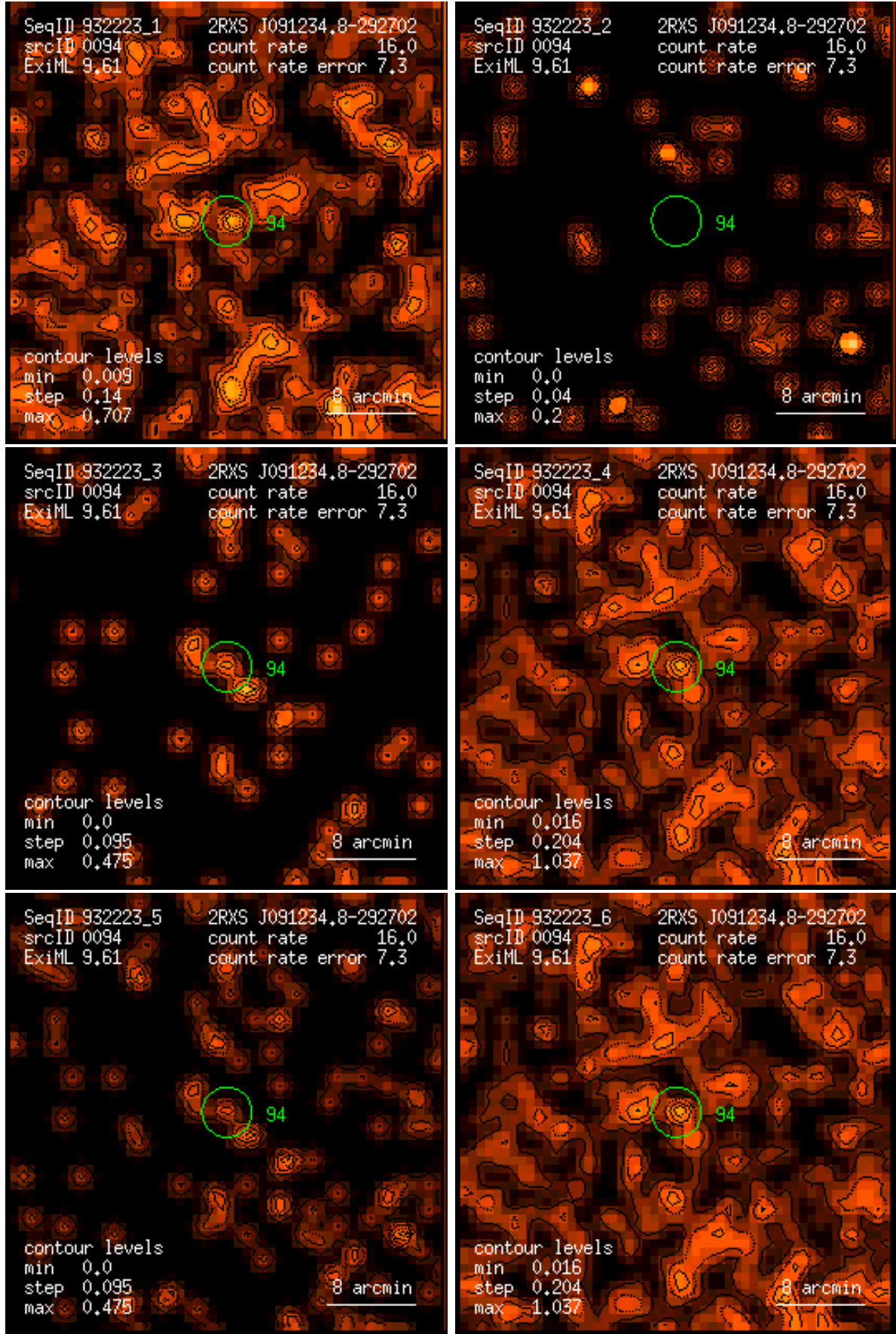
Figure 94: RASS 932223: detection 0094: band rate images, Gaussian filter: (1) PSPC channels 11 – 41, (2) 52 – 90, (3) 91 – 201, (4) 11 – 235, (5) 52 – 201, (6) 11 – 201. Broad band rates in counts/ks. Band rate contour levels in counts/ks/arcmin 2 .
