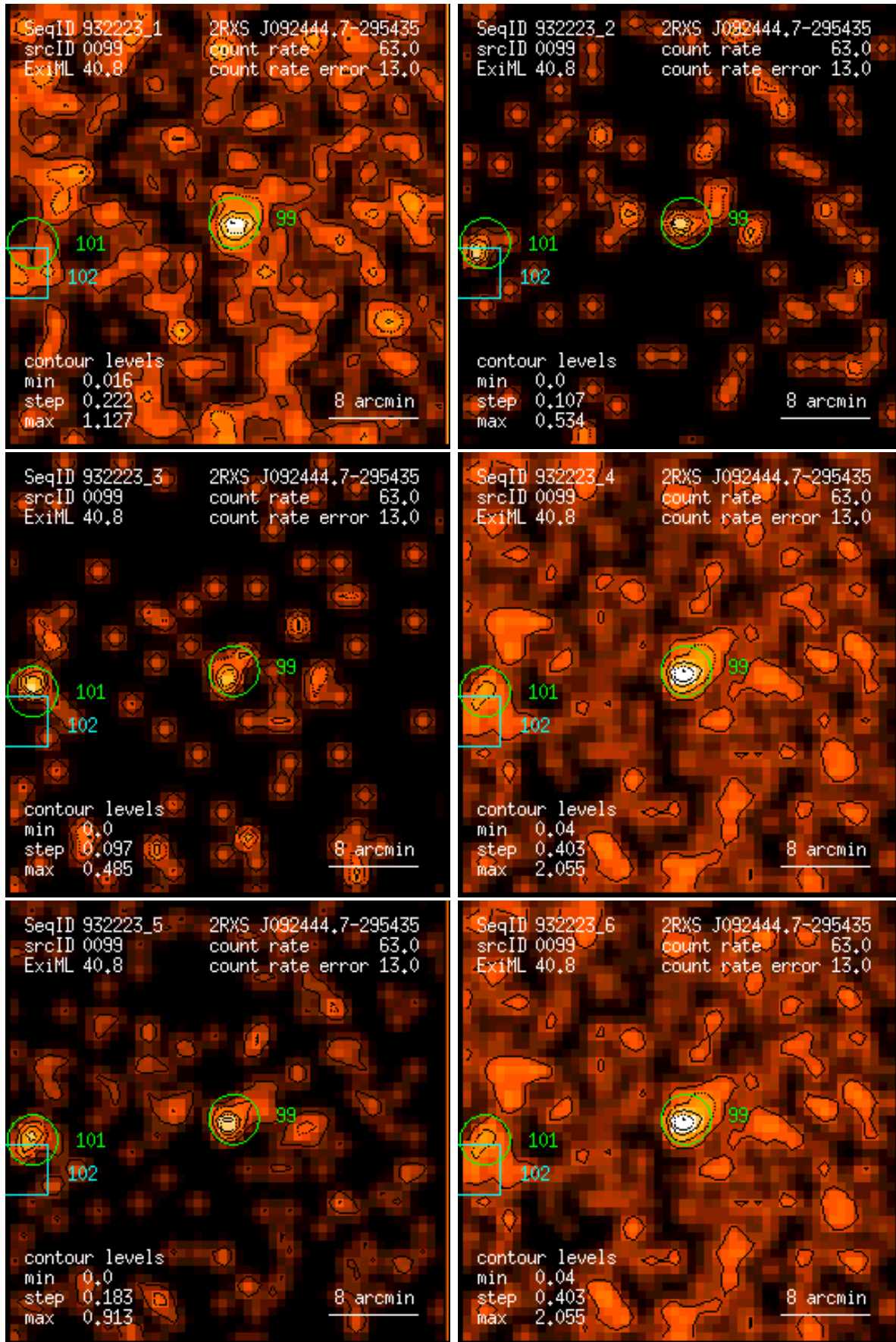
Figure 99: RASS 932223: detection 0099: band rate images, Gaussian filter: (1) PSPC channels 11 – 41, (2) 52 – 90, (3) 91 – 201, (4) 11 – 235, (5) 52 – 201, (6) 11 – 201. Broad band rates in counts/ks. Band rate contour levels in counts/ks/arcmin 2 .
