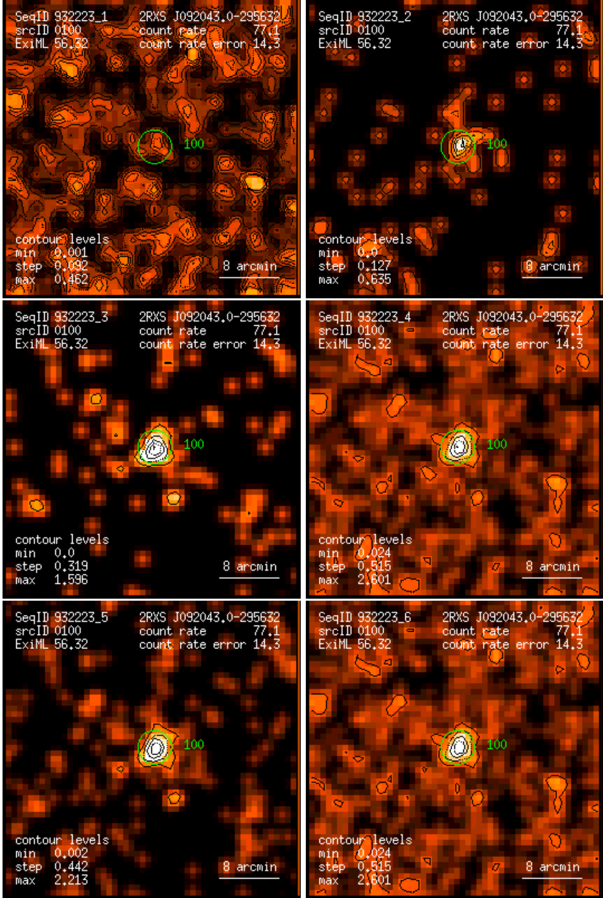
Figure 100: RASS 932223: detection 0100: band rate images, Gaussian filter: (1) PSPC channels 11 – 41, (2) 52 – 90, (3) 91 – 201, (4) 11 – 235, (5) 52 – 201, (6) 11 – 201. Broad band rates in counts/ks. Band rate contour levels in counts/ks/arcmin 2 .
