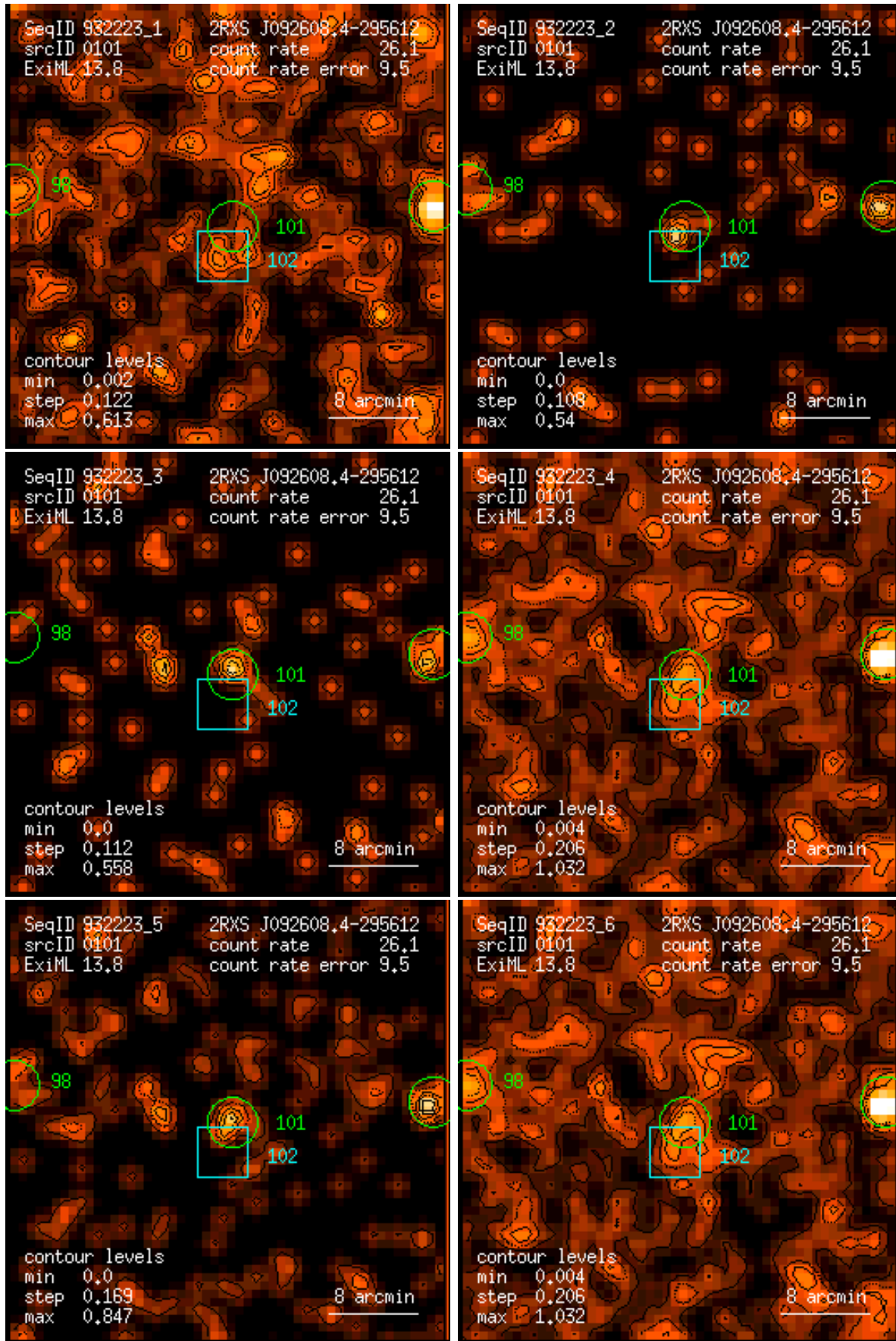
Figure 101: RASS 932223: detection 0101: band rate images, Gaussian filter: (1) PSPC channels 11 – 41, (2) 52 – 90, (3) 91 – 201, (4) 11 – 235, (5) 52 – 201, (6) 11 – 201. Broad band rates in counts/ks. Band rate contour levels in counts/ks/arcmin 2 .
