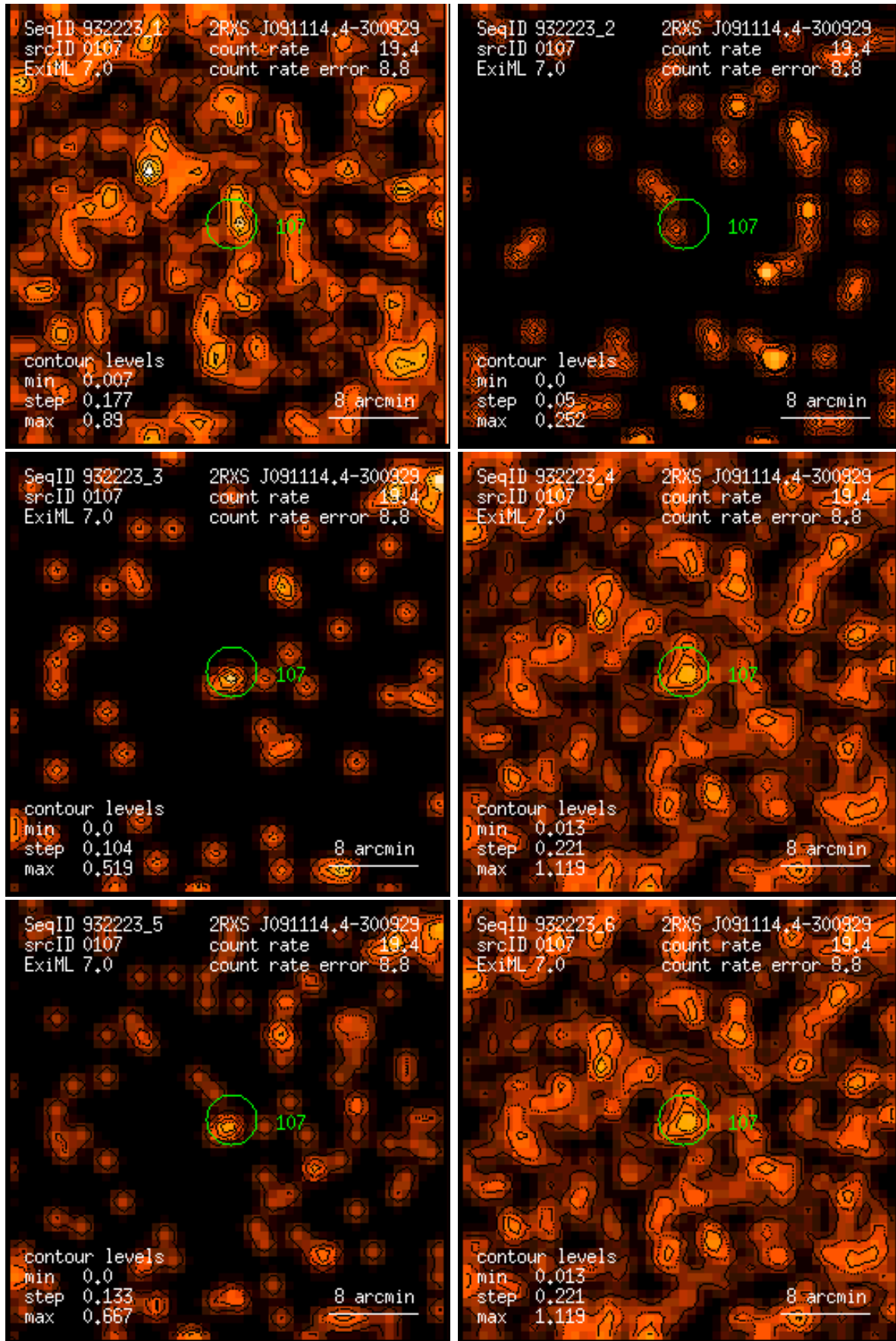
Figure 107: RASS 932223: detection 0107: band rate images, Gaussian filter: (1) PSPC channels 11 – 41, (2) 52 – 90, (3) 91 – 201, (4) 11 – 235, (5) 52 – 201, (6) 11 – 201. Broad band rates in counts/ks. Band rate contour levels in counts/ks/arcmin 2 .
