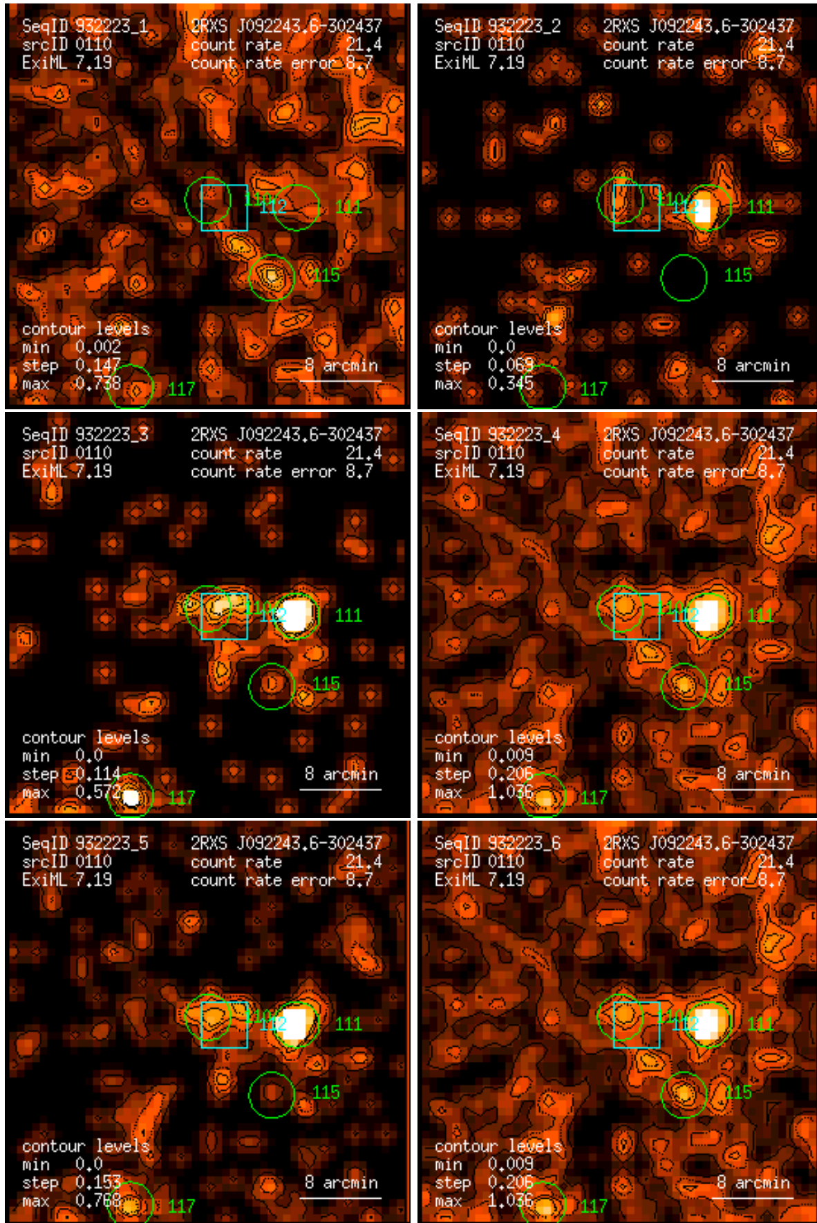
Figure 110: RASS 932223: detection 0110: band rate images, Gaussian filter: (1) PSPC channels 11 – 41, (2) 52 – 90, (3) 91 – 201, (4) 11 – 235, (5) 52 – 201, (6) 11 – 201. Broad band rates in counts/ks. Band rate contour levels in counts/ks/arcmin 2 .
