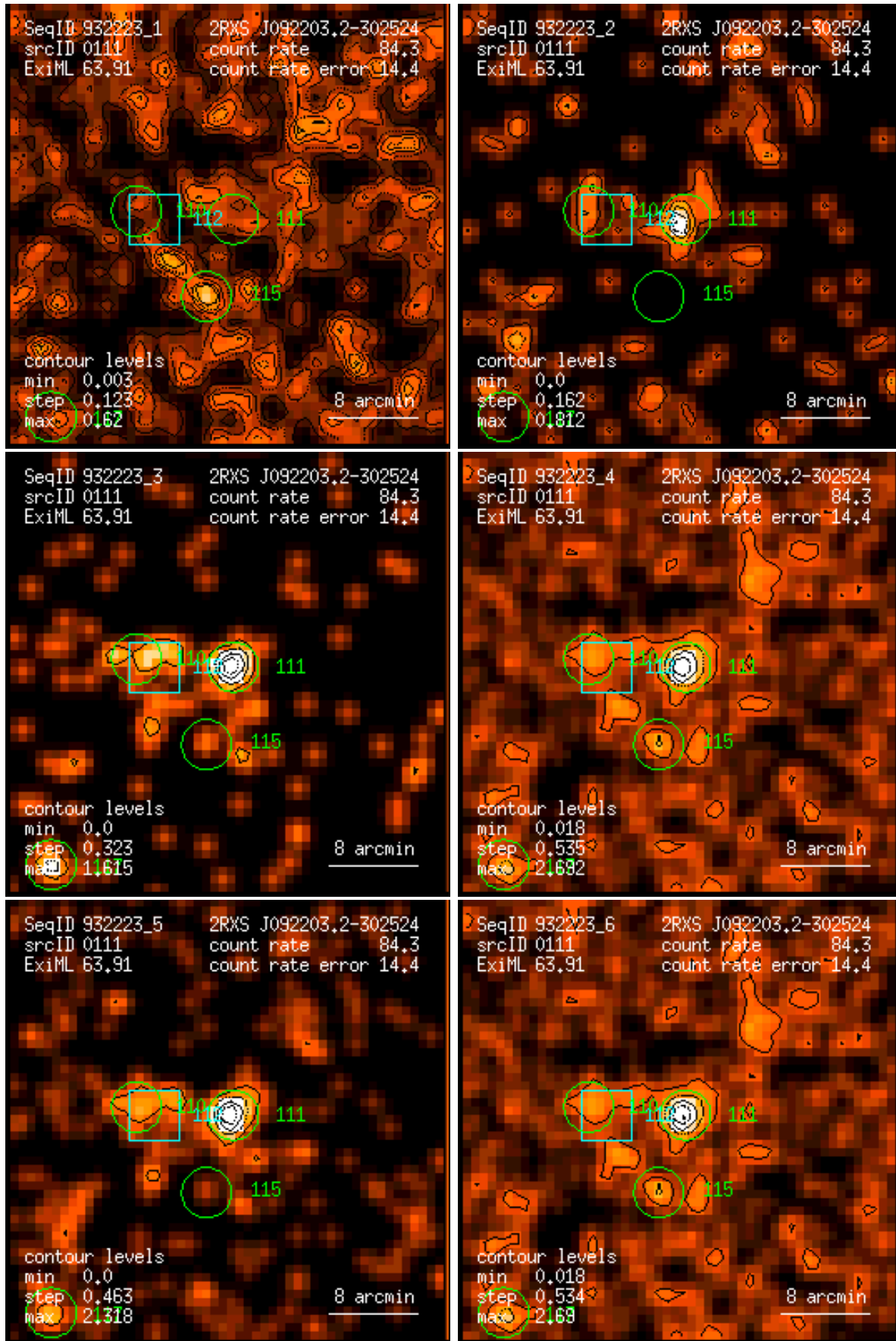
Figure 111: RASS 932223: detection 0111: band rate images, Gaussian filter: (1) PSPC channels 11 – 41, (2) 52 – 90, (3) 91 – 201, (4) 11 – 235, (5) 52 – 201, (6) 11 – 201. Broad band rates in counts/ks. Band rate contour levels in counts/ks/arcmin 2 .
