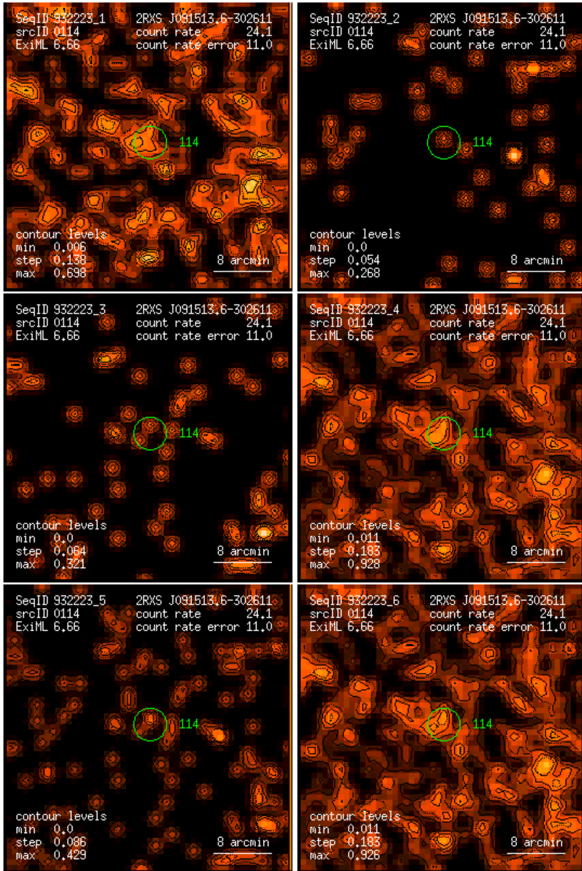
Figure 114: RASS 932223: detection 0114: band rate images, Gaussian filter: (1) PSPC channels 11 – 41, (2) 52 – 90, (3) 91 – 201, (4) 11 – 235, (5) 52 – 201, (6) 11 – 201. Broad band rates in counts/ks. Band rate contour levels in counts/ks/arcmin 2 .
