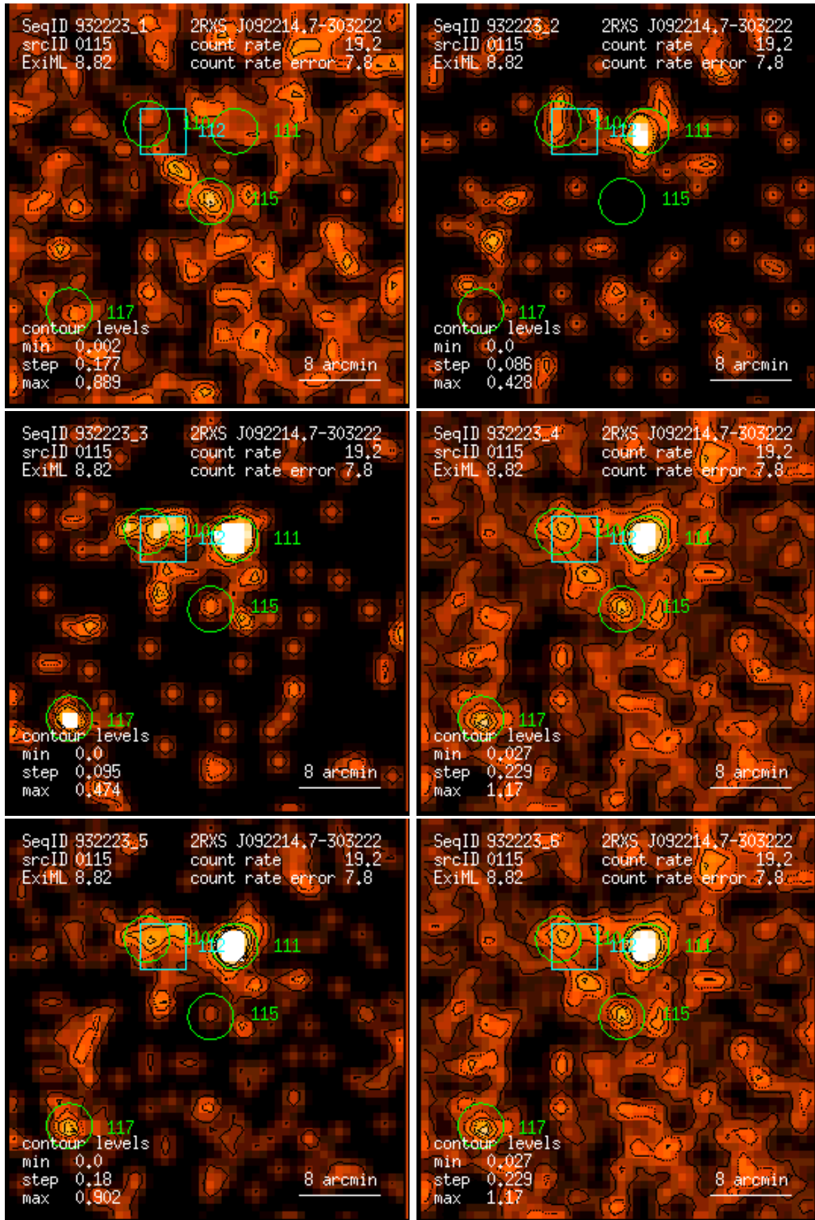
Figure 115: RASS 932223: detection 0115: band rate images, Gaussian filter: (1) PSPC channels 11 – 41, (2) 52 – 90, (3) 91 – 201, (4) 11 – 235, (5) 52 – 201, (6) 11 – 201. Broad band rates in counts/ks. Band rate contour levels in counts/ks/arcmin 2 .
